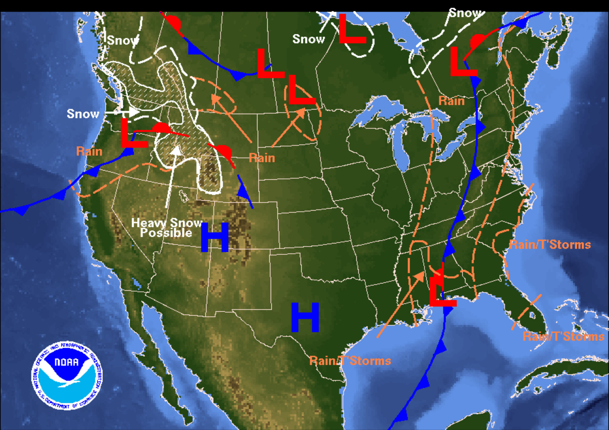
Weather Forecast for Tuesday, November 01, 2005 DOC/NOAA/NWS/NCEP/Hydrometeorological Prediction Center Prepared by Bell/Terry based on HPC, SPC, and TPC forecasts.
