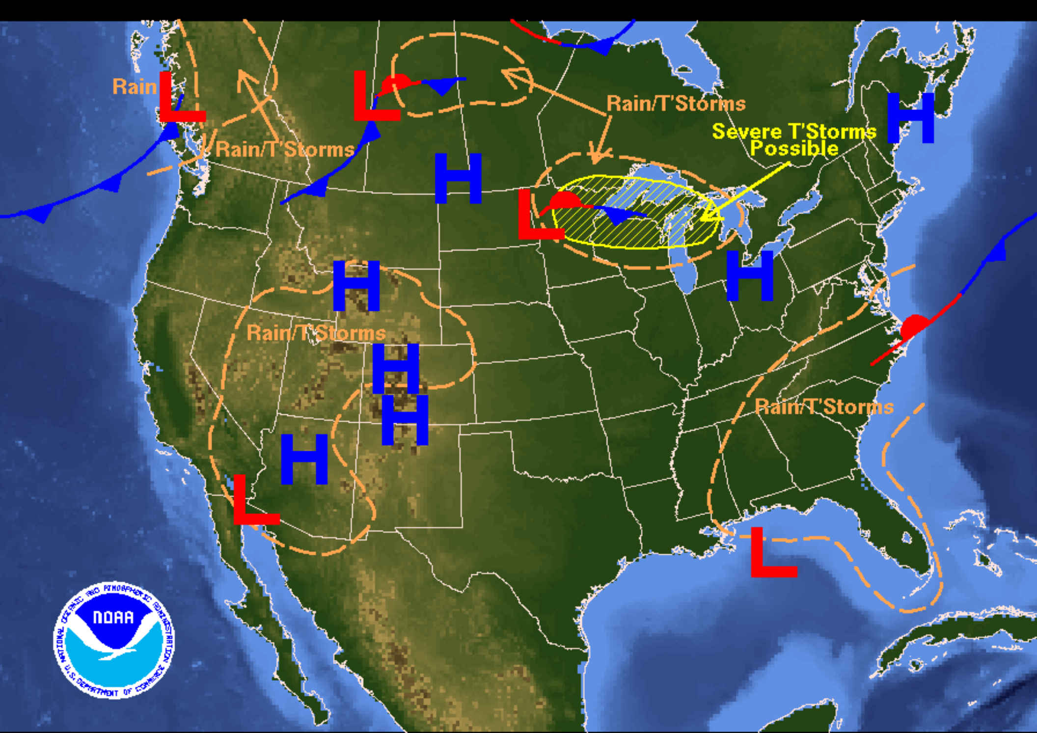
Weather Forecast for Sunday, July 31, 2005 DOC/NOAA/NWS/NCEP/Hydrometeorological Prediction Center Prepared by Halbach/Sullivan based on HPC, SPC, and TPC forecasts.
