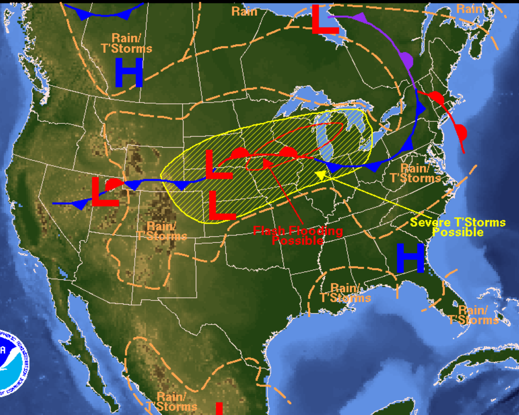
Weather Forecast for Monday, July 25, 2005 DOC/NOAA/NWS/NCEP/Hydrometeorological Prediction Center Prepared by Fries/Korty based on HPC, SPC, and TPC forecasts.
