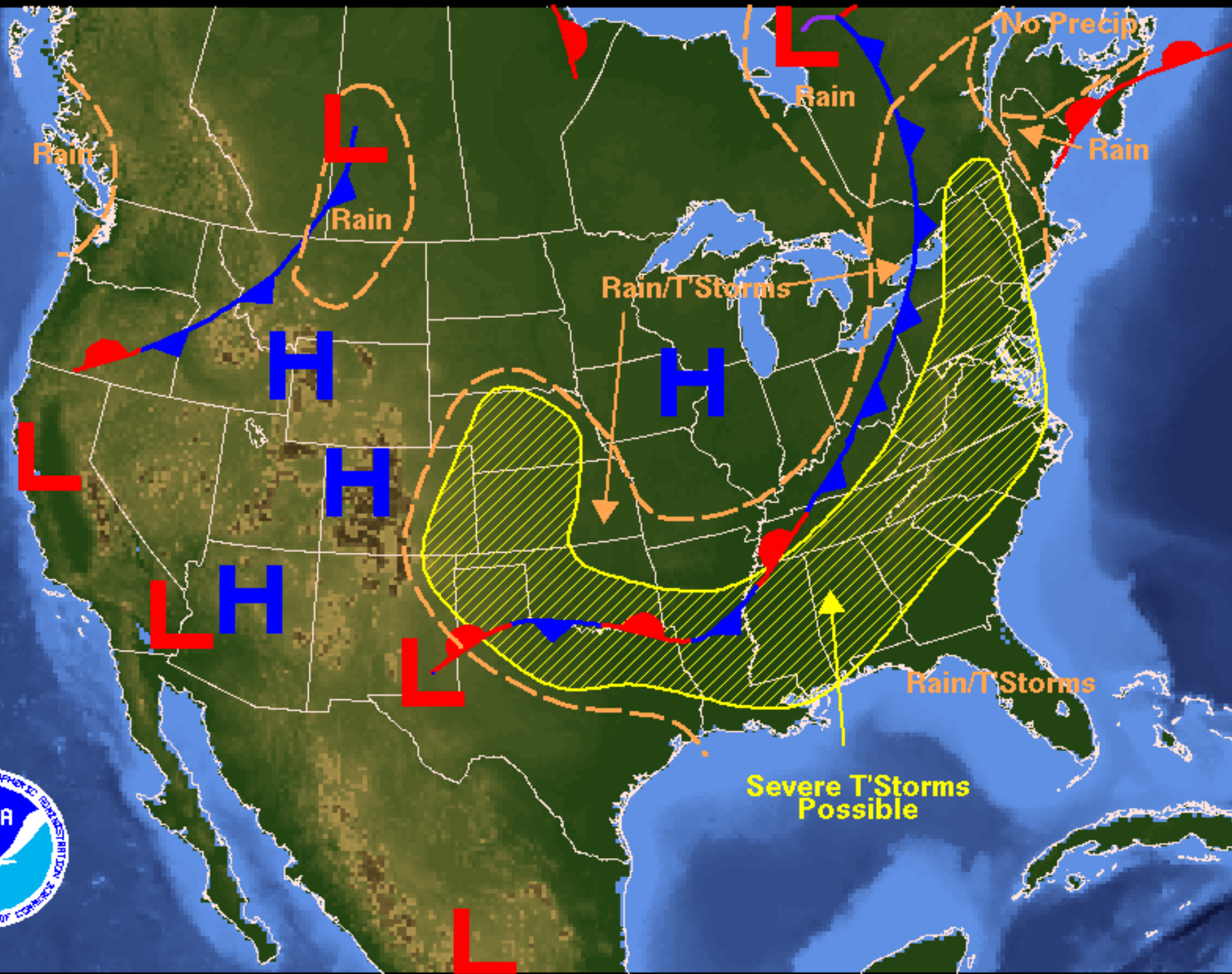
Weather Forecast for Friday, July 01, 2005 DOC/NOAA/NWS/NCEP/Hydrometeorological Prediction Center Prepared by SzataneK/Oravec based on HPC, SPC, and TPC forecasts.
