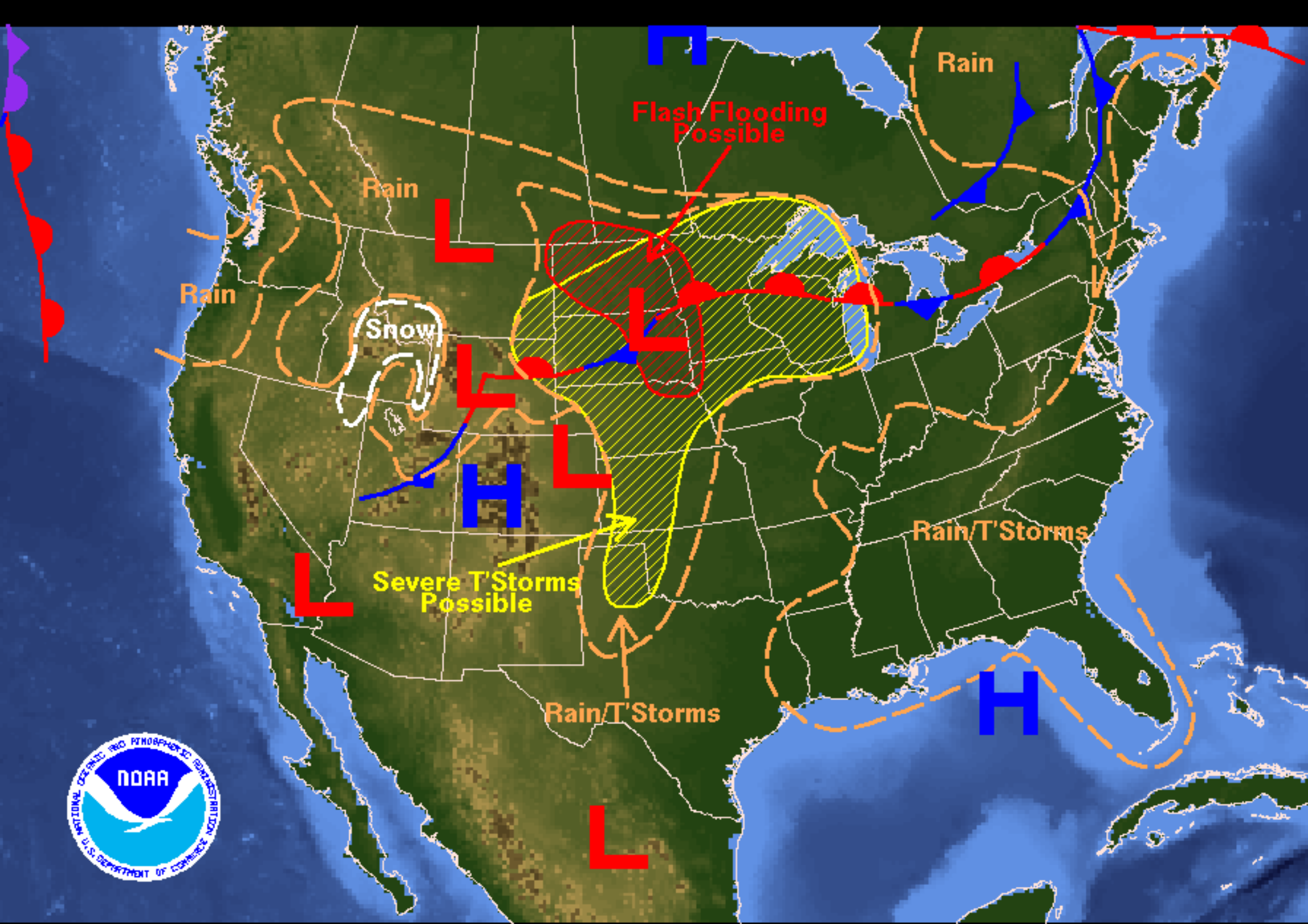
Weather Forecast for Tuesday, June 07, 2005 DOC/NOAA/NWS/NCEP/Hydrometeorological Prediction Center Prepared by Halbach/Eckert based on HPC, SPC, and TPC forecasts.
