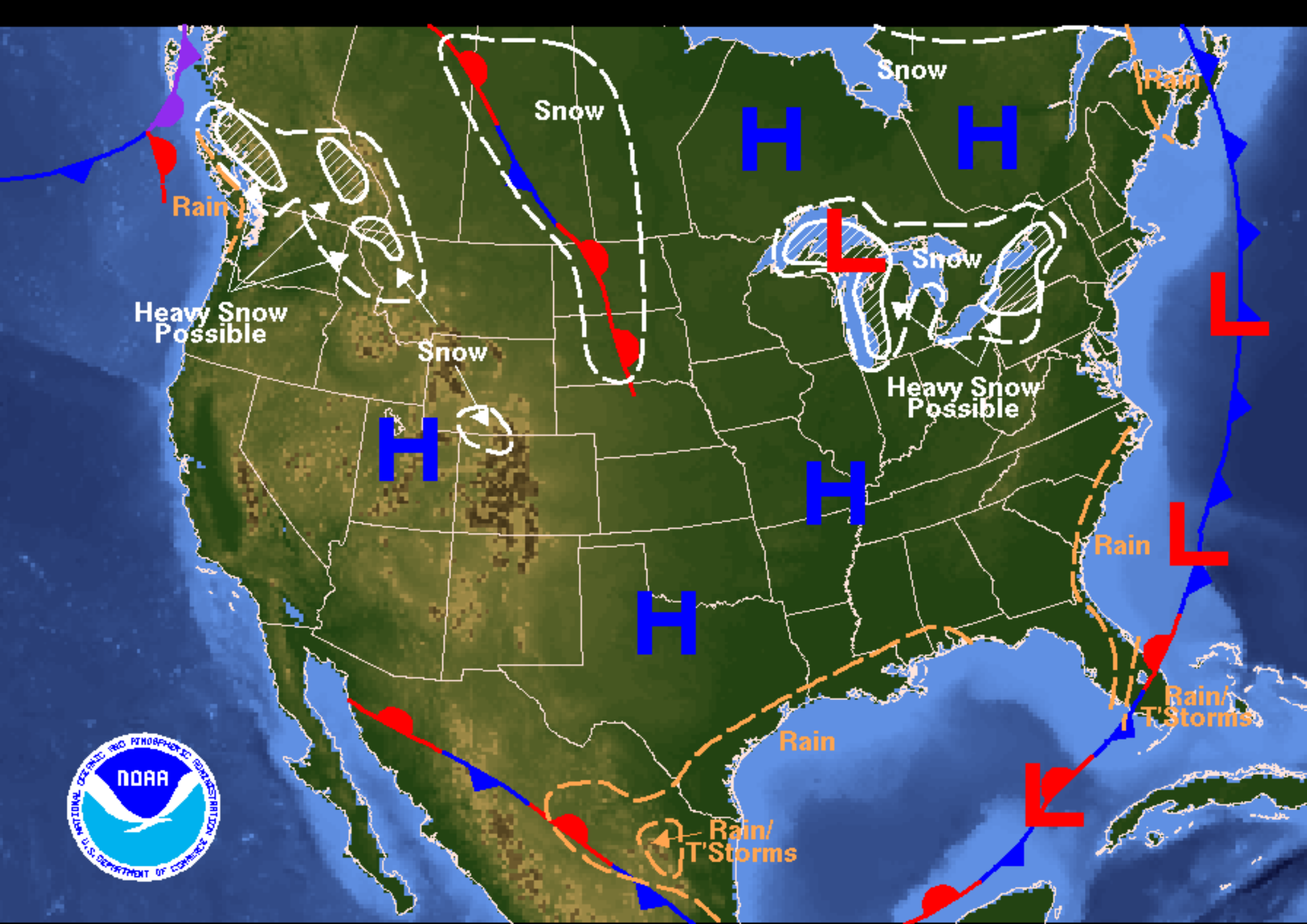
Weather Forecast for Friday, December 24, 2004 DOC/NOAA/NWS/NCEP/Hydrometeorological Prediction Center Prepared by SzataneK/Korty based on HPC, SPC, and TPC forecasts.
