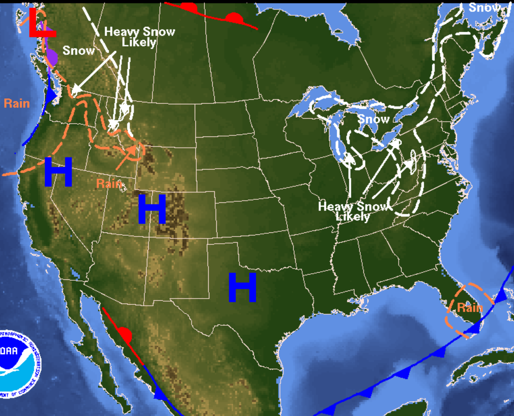
Weather Forecast for Tuesday, December 14, 2004 DOC/NOAA/NWS/NCEP/Hydrometeorological Prediction Center Prepared by Bell/Eckert based on HPC, SPC, and TPC forecasts.
