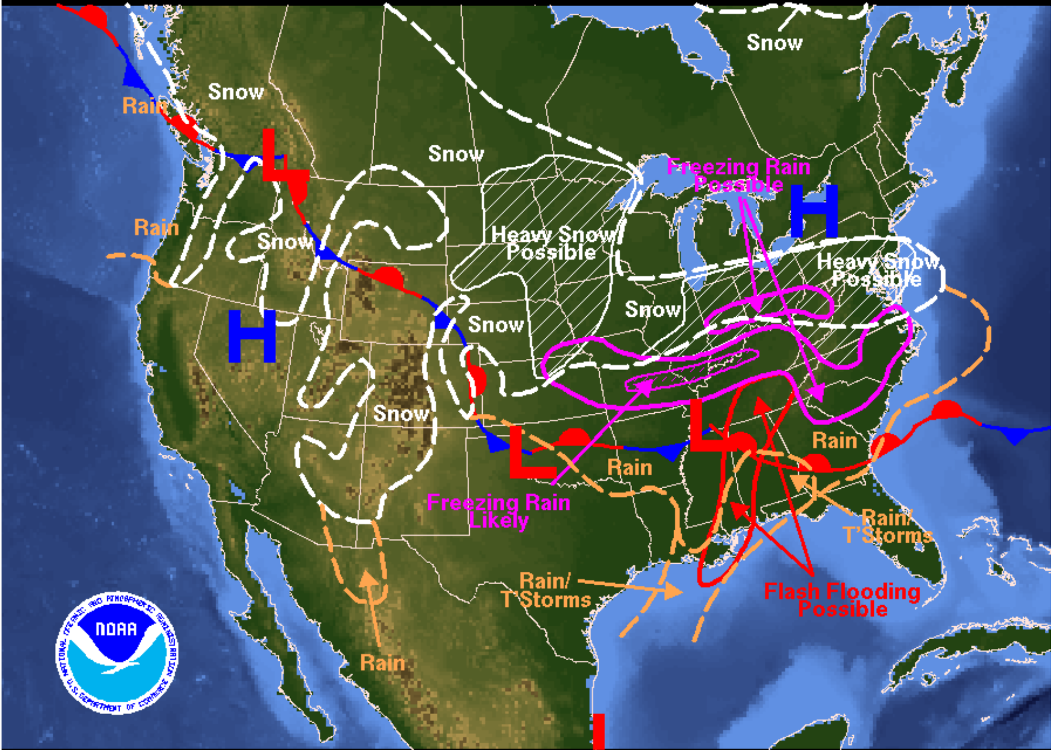
Weather Forecast for Sunday, January 25, 2004 DOC/NOAA/NWS/NCEP/Hydrometeorological Prediction Center Prepared by Hatchett/Oravec based on HPC, SPC, and TPC forecasts.
