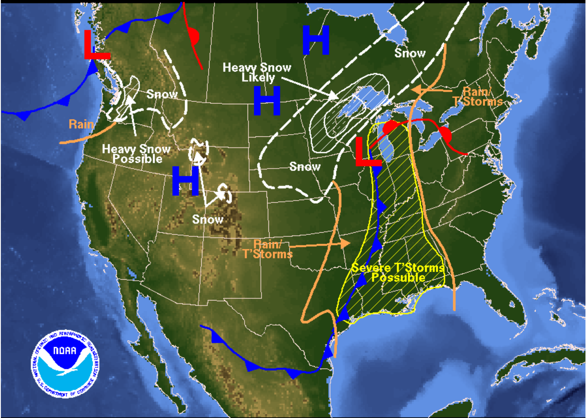
Weather Forecast for Sunday, November 23, 2003 DOC/NOAA/NWS/NCEP/Hydrometeorological Prediction Center Prepared by Hatchett/Eckert based on HPC, SPC, and TPC forecasts.
