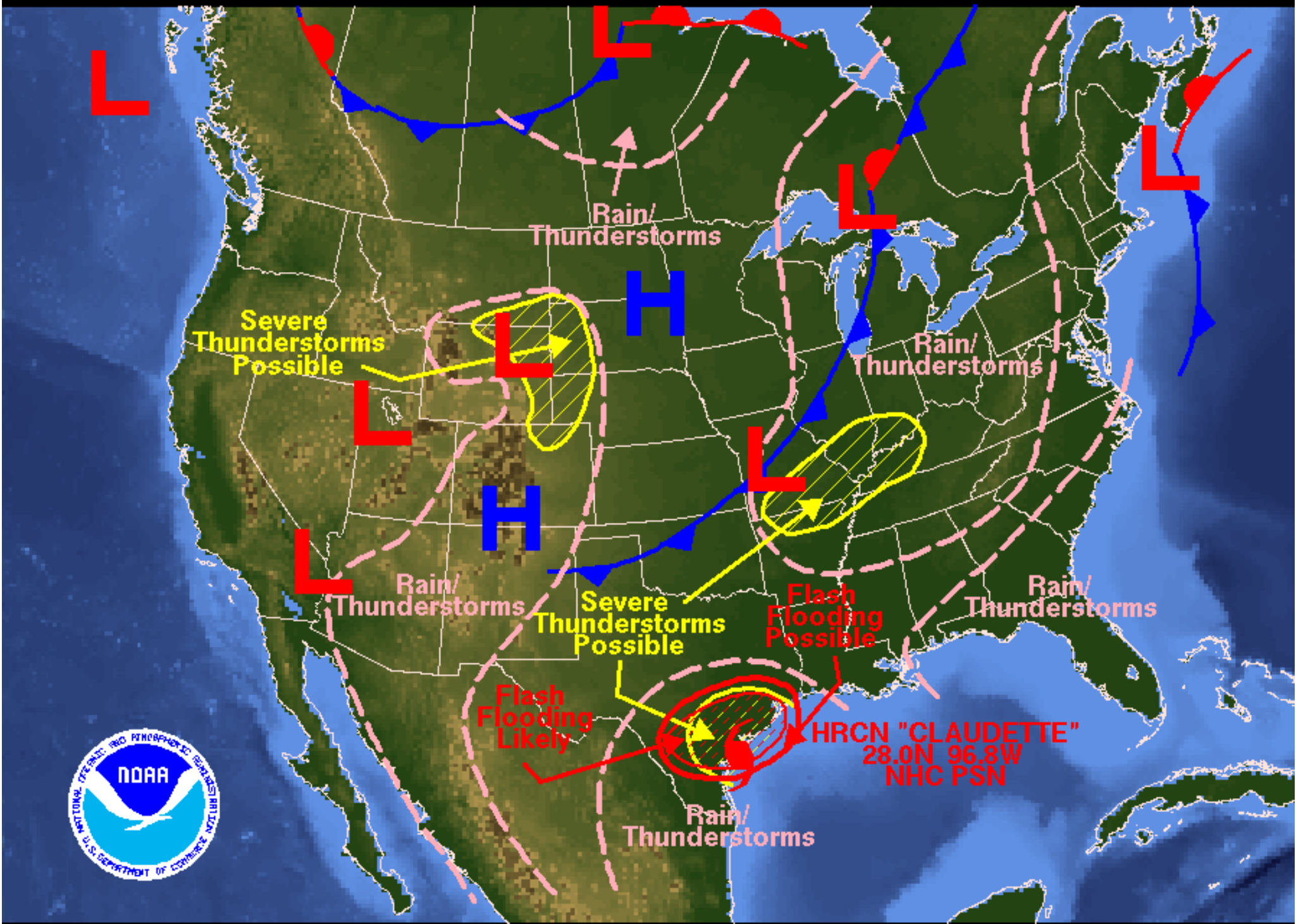
Weather Forecast for Tuesday, July 15, 2003 DOC/NOAA/NWS/NCEP/Hydrometeorological Prediction Center Prepared by Hatchett/Terry based on HPC, SPC, and TPC forecasts.
