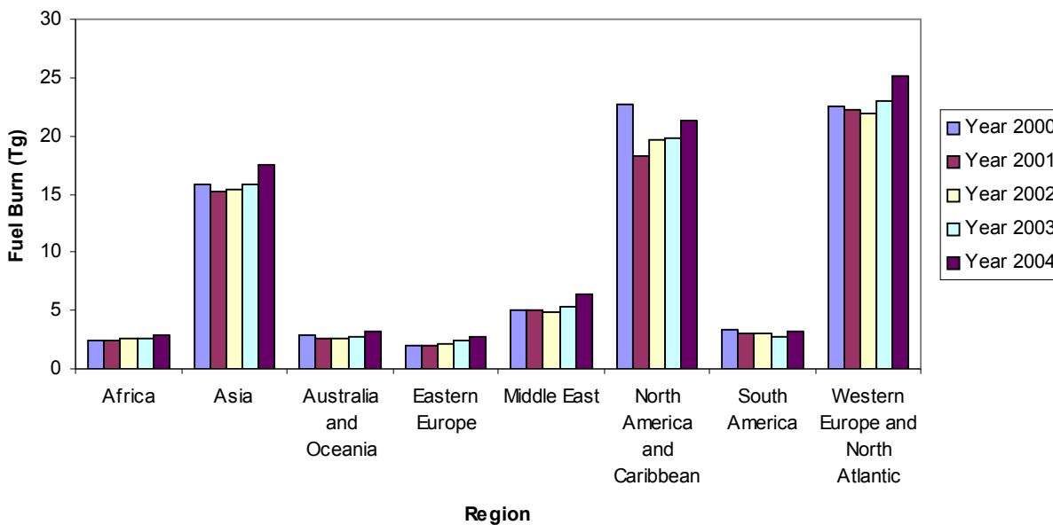
Figure 5. Comparison of Regional International Fuel Burn
