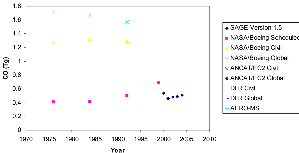
Figure 22. Comparison of CO Emissions from Past Studies
