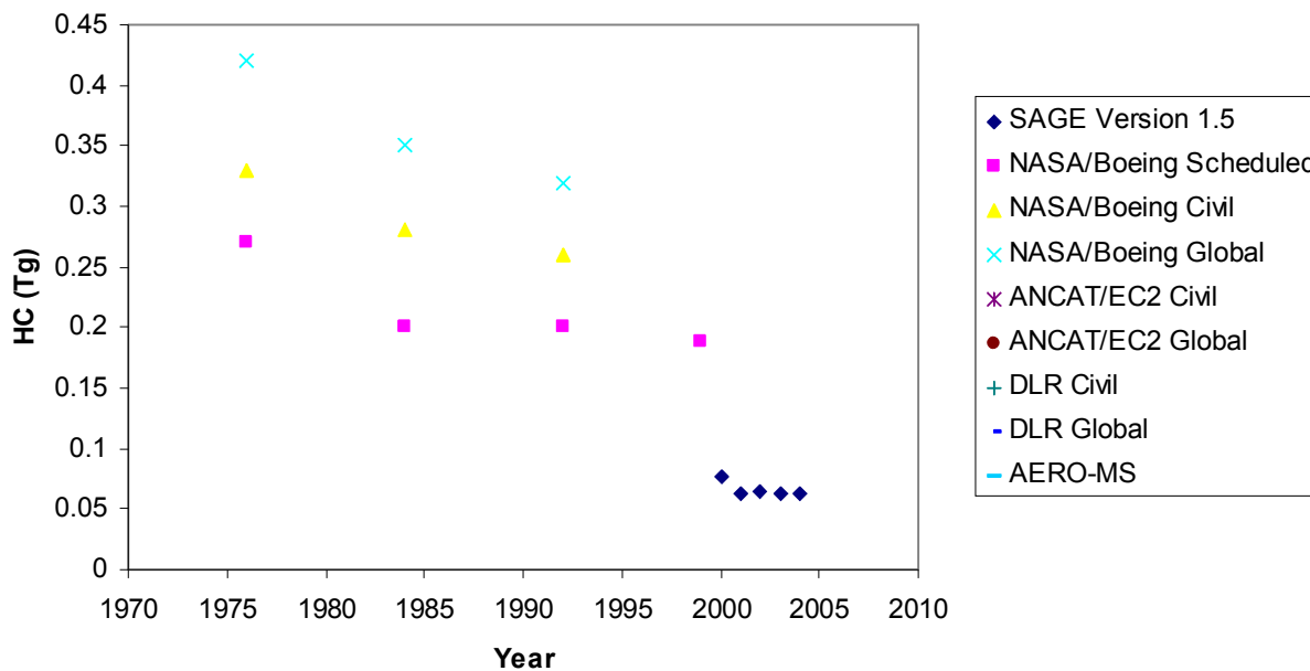
Figure 23. Comparison of HC Emissions from Past Studies
