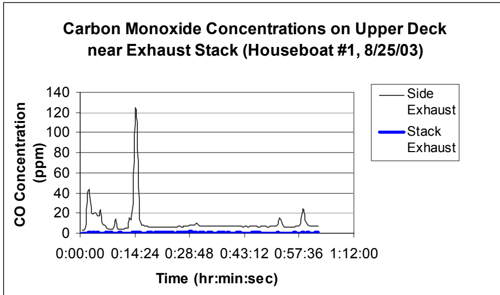
Figure 7. Comparison of CO concentrations on the upper level of houseboat #1 near the exhaust stack. (under conditions of no generator load and no extra weight).
