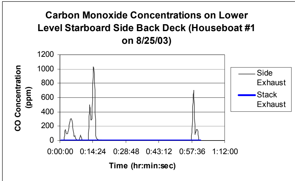
Figure 5. Comparison of CO concentrations on the lower level starboard side back deck of houseboat #1 (side exhaust was located on starboard rear side of boat at water level). Under conditions of no generator load and no extra weight.
