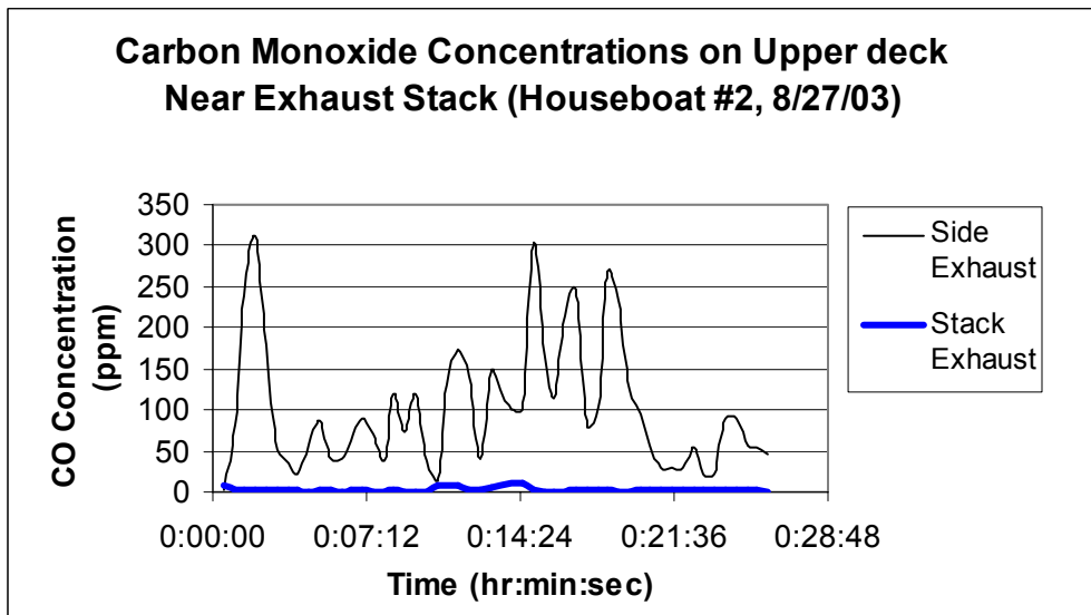
Figure 8. Comparison of CO concentrations on the upper level of houseboat #2 near the exhaust stack. (under conditions of no generator load and no extra weight).
