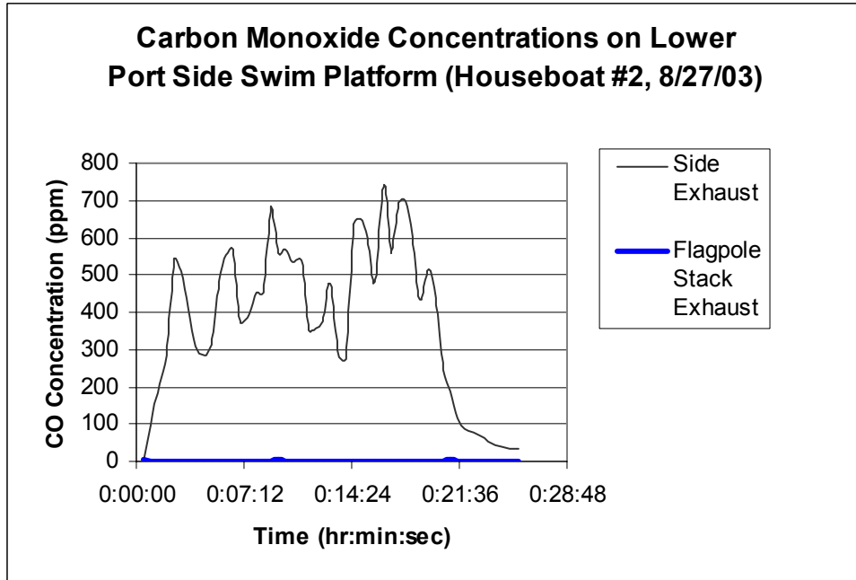
Figure 6. Comparison of CO concentrations on the lower level port side swim platform of houseboat #2 (side exhaust was located on port rear side of boat at water level). Under conditions of no generator load and no extra weight.
