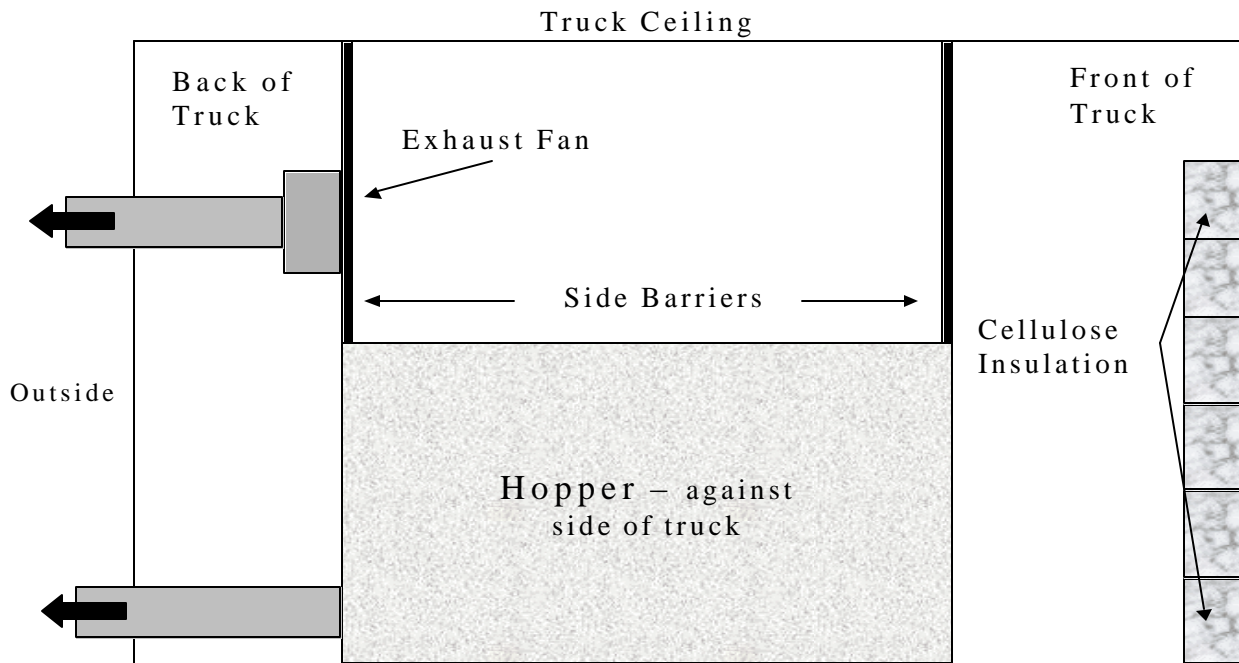
Figure 2. Proposed engineering control (#2) for hopper area.
