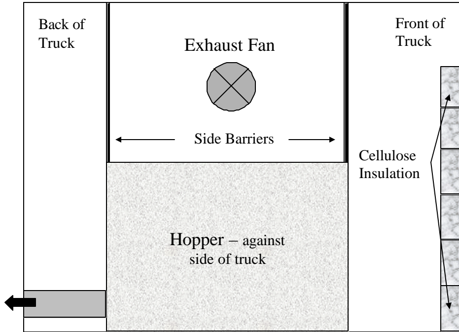
Figure 1. Proposed engineering control for hopper area.
