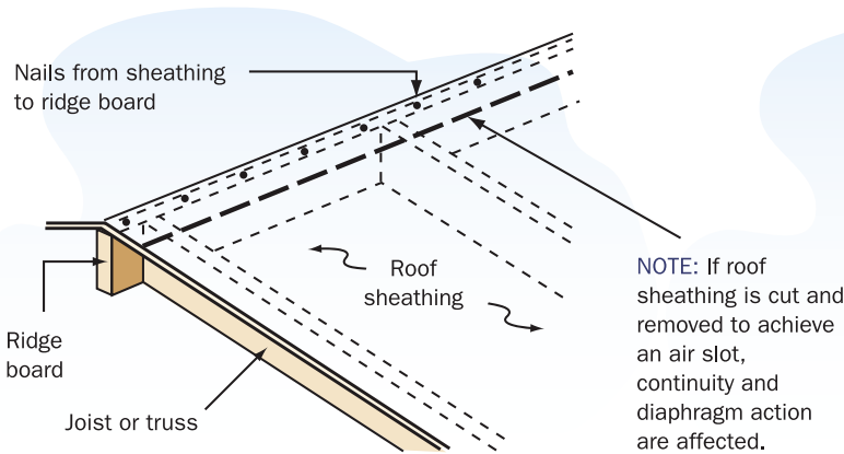
Method for maintaining a continuous load path at the roof ridge by nailing roof sheathing.
