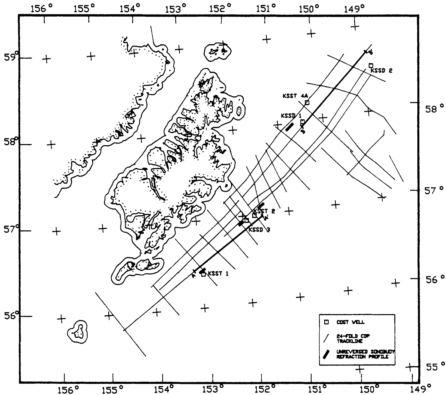
Figure 46. Map showing trackline coverage of 24-fold seismic reflection profile data across Kodiak shelf. Also shown are the locations of unreversed sonobuoy refraction profiles shot near wells.
