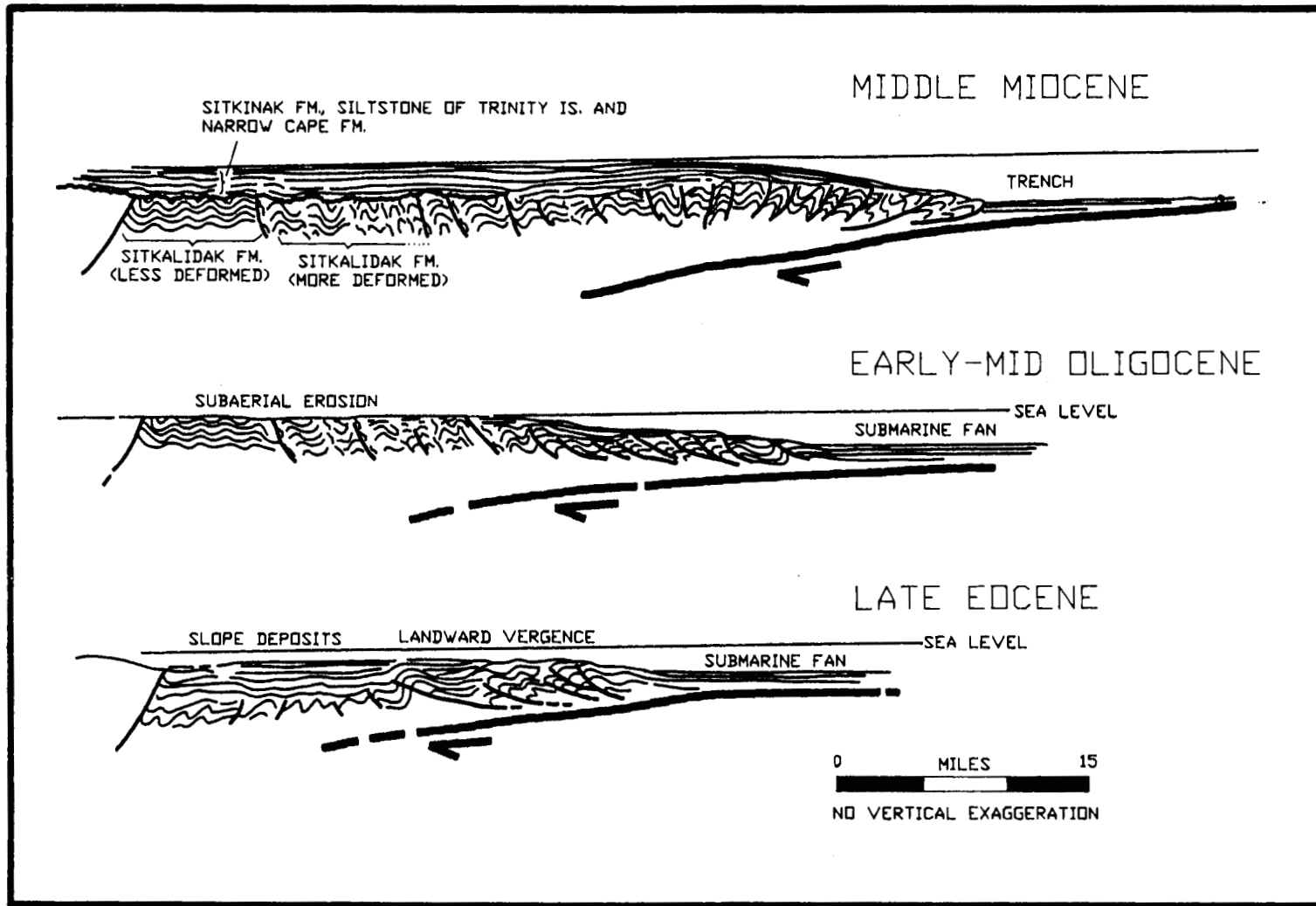
Figure 56. Tectonic evolution of the Kodiak shelf (after Moore and Allwardt, 1980) illustrating the development of the more deformed and less deformed units of the Sitkalidak formation.
