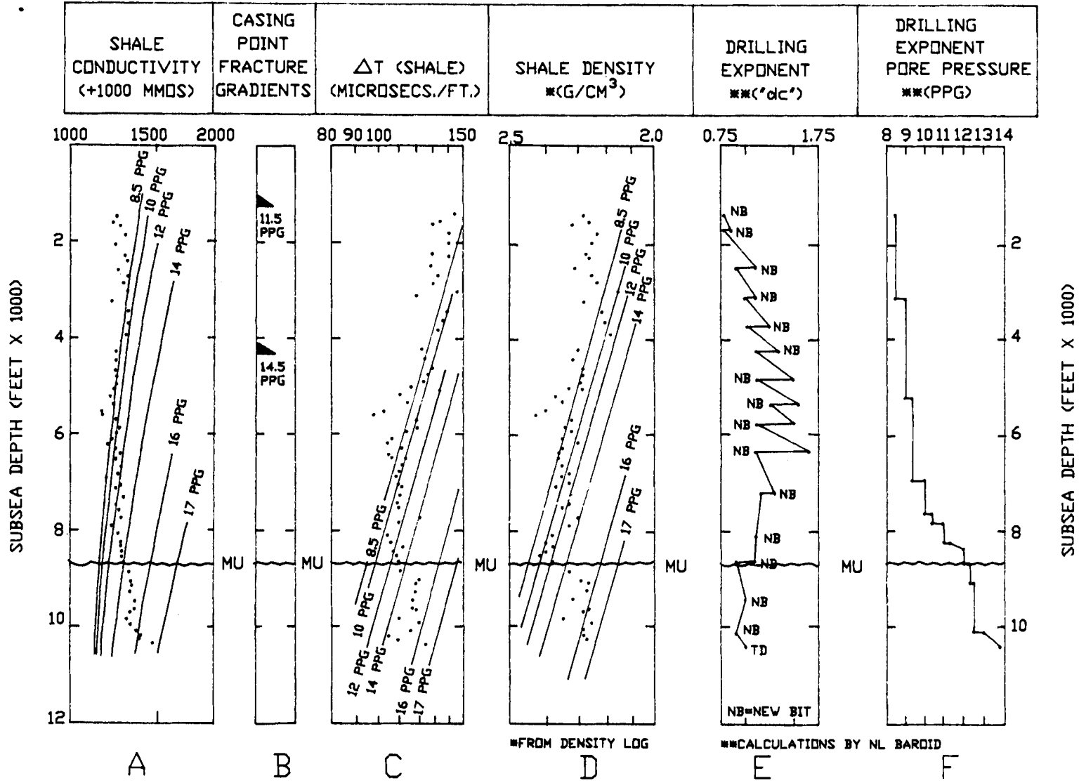
Figure 90. Sun Oil KSSD No. 2 well. Synopsis of drilling data and wireline log data for shales. Normal compaction trends can be identified in the interval from 3,400 to 6,500 feet. Strata below 6,500 feet appear to be overpressured.
