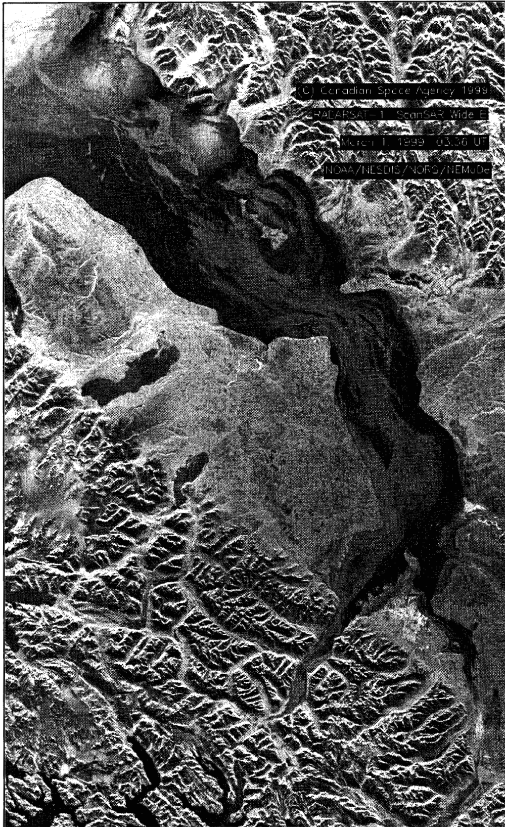
Figure 28. RADARSAT SAR image on middle and upper Cook Inlet, 1 March 1999 showing extensive ice coverage.
