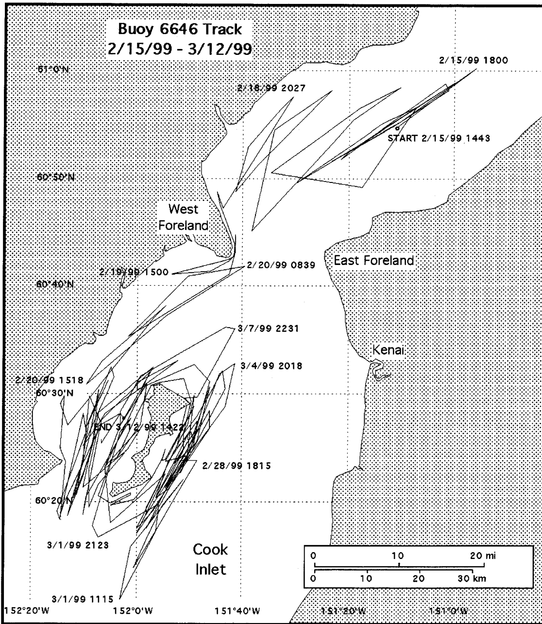
Figure 29. Buoy 6646 track, 15 February 1999 to 12 March 1999.
