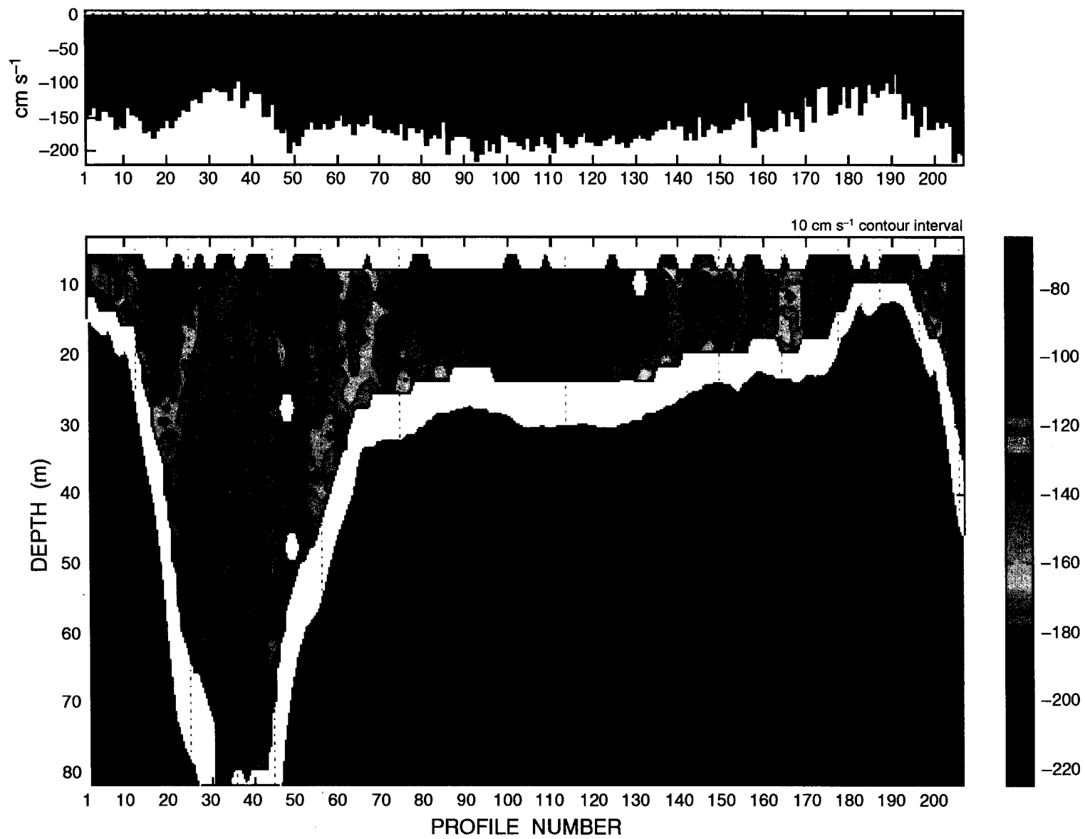
Figure 3. North-south velocity, section 20 CIRCAC Cook Inlet data, 11:10-14:38 AST, 18 June 1999.
