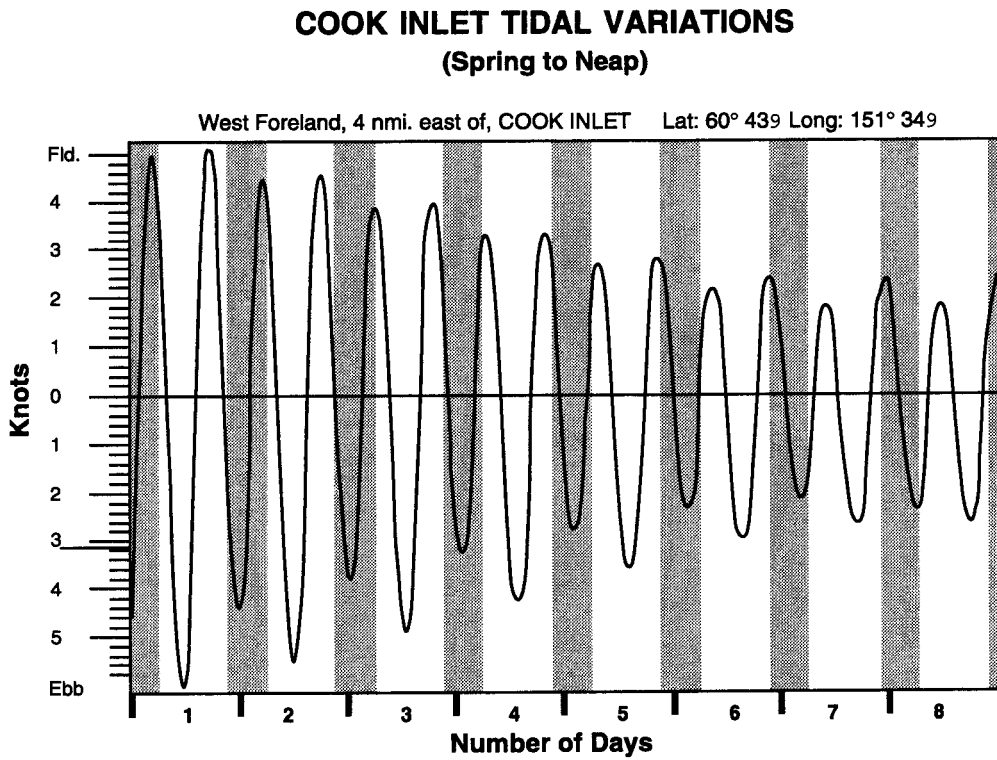
Figure 6. Cook Inlet tidal current variations.
