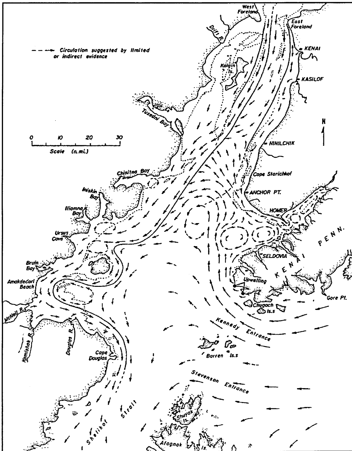
Figure 2. Net surface circulation in lower Cook Inlet, based primarily on data collected during the spring and summer seasons [Burbank 1977].
