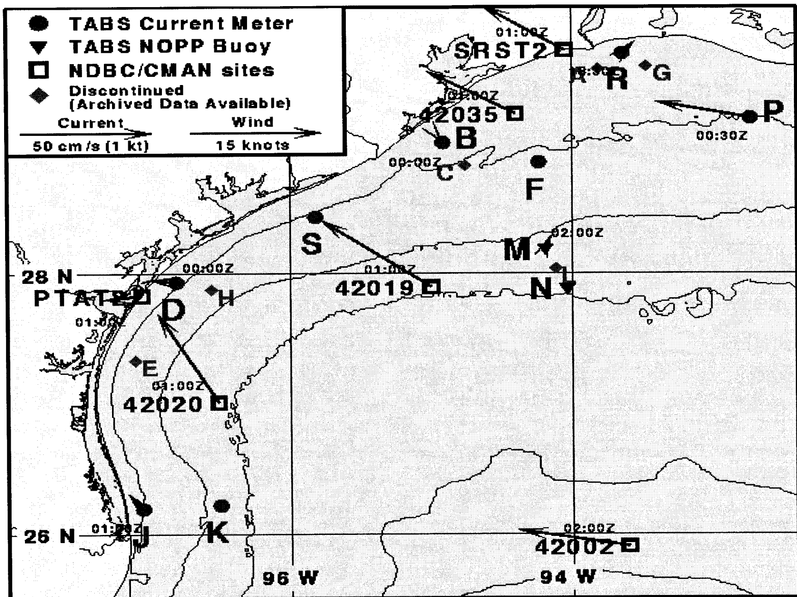
Figure 2. TABS Gulf of Mexico measurement array.
