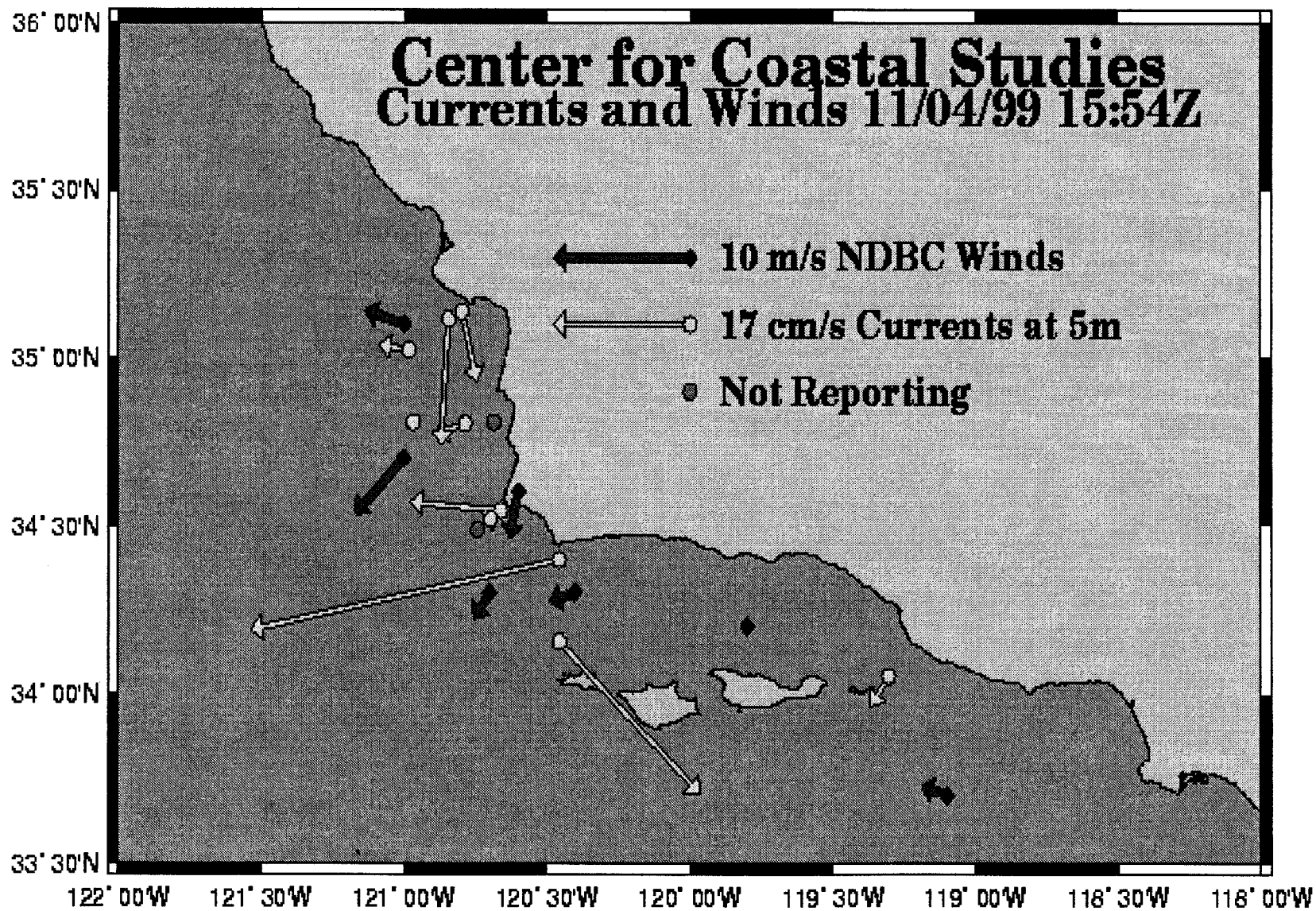
Figure 3. Observed data for the Santa Barbara Channel.
