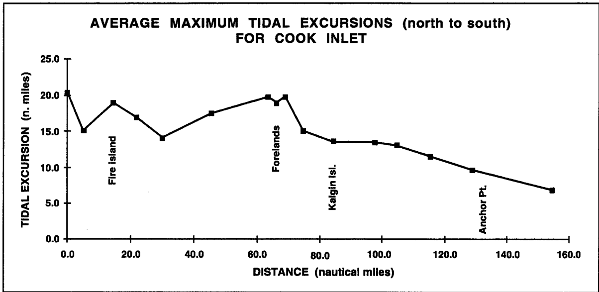
Figure 7. Average maximum tidal excursions for Cook Inlet.
