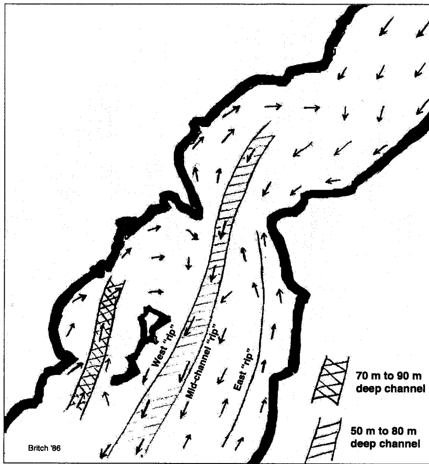
Figure 8. Middle Cook Inlet circulation and convergence zones.
