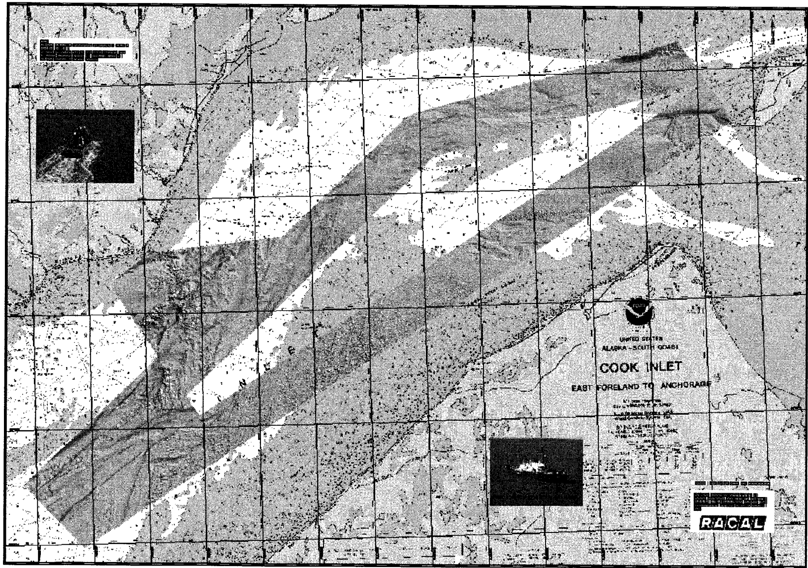
Figure 1. Summer 1999 sonar image of upper Cook Inlet bathymetry.
