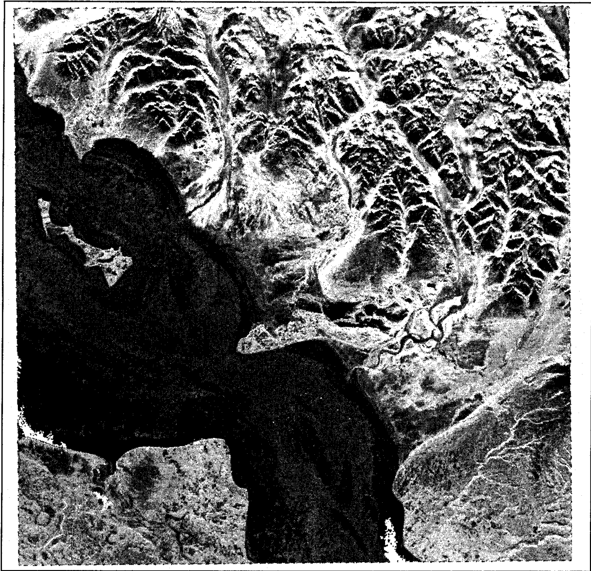
Figure 27. RADARSAT SAR image of middle Cook Inlet, 15 February 1999, showing 8/10 to 9/10 ice coverage. Dark, non-reflective returns from the west side of Cook Inlet are not open water, but sea ice covered with a smooth layer of snow.
