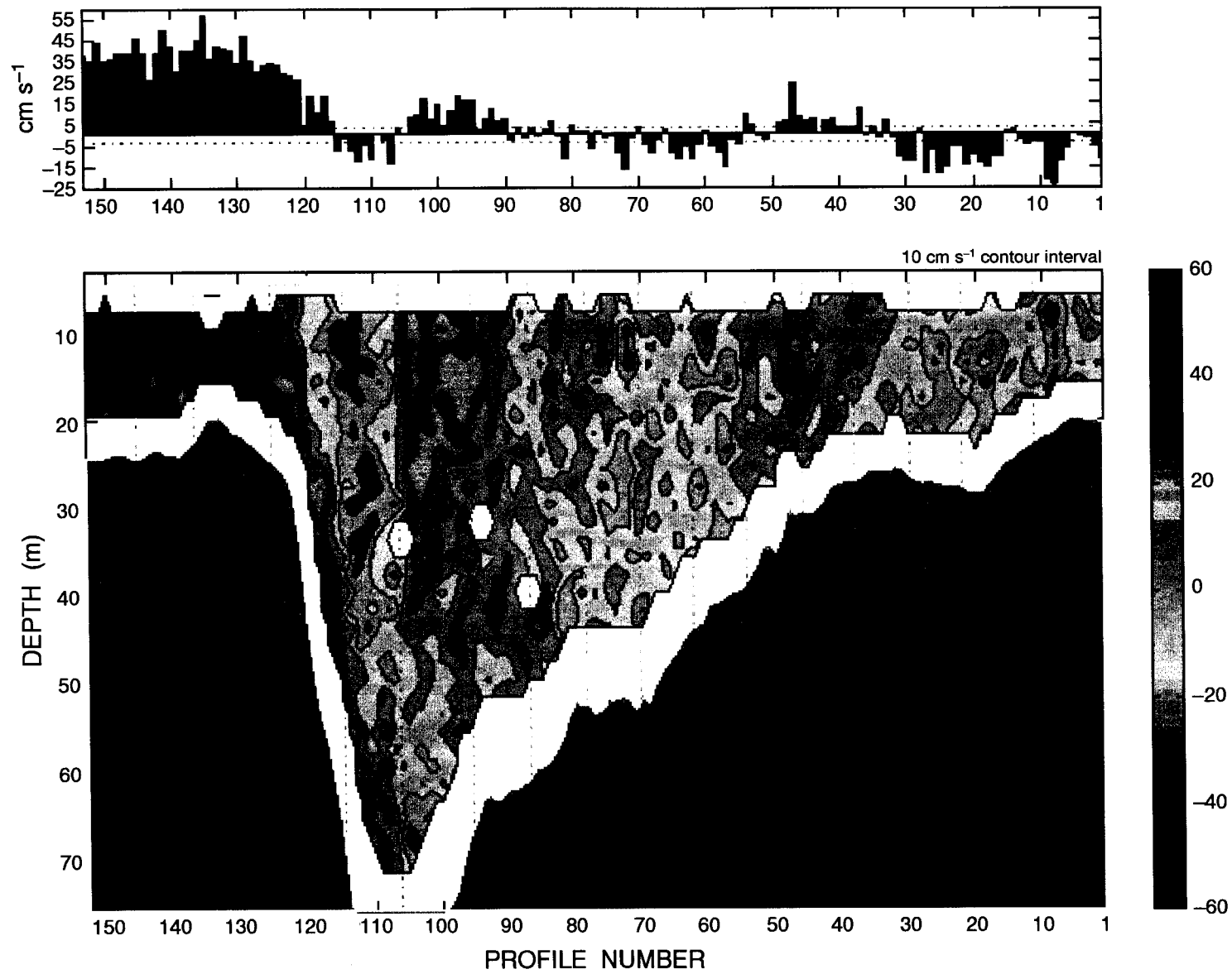
Figure 5. East-west velocity, section 12 CIRCAC Cook Inlet data, 19:38–21:43 AST, 17 June 1999.
