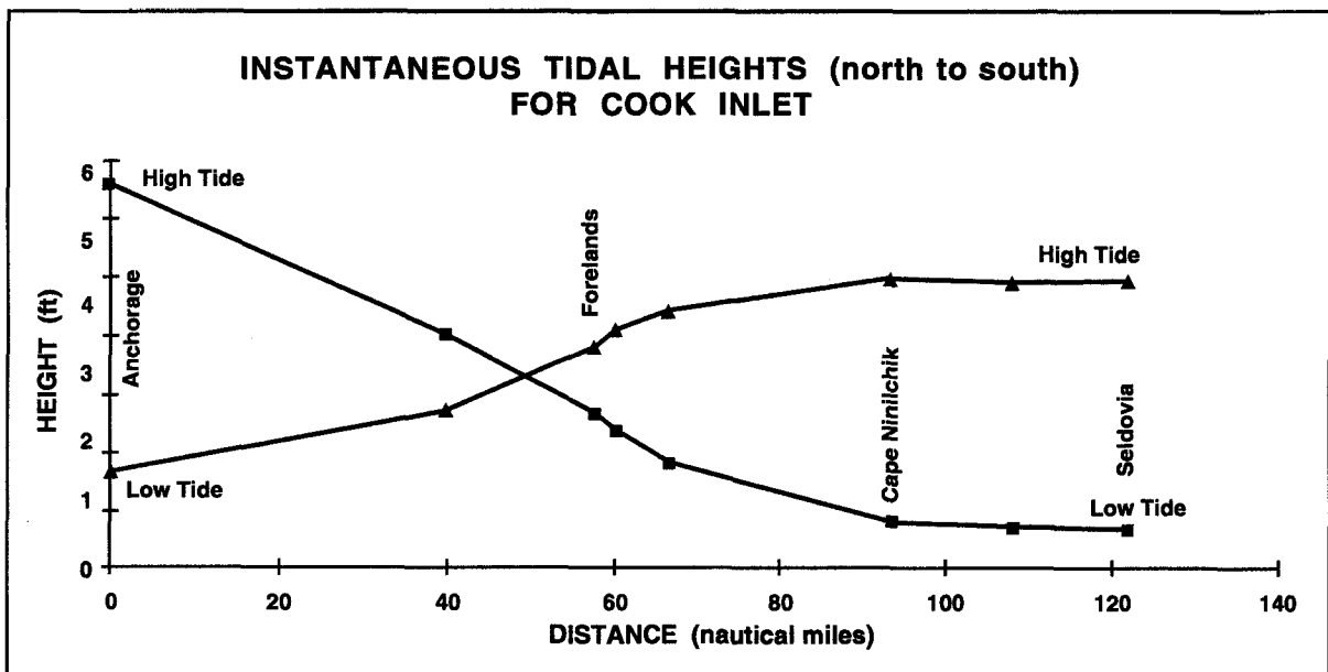
Figure 4. Instantaneous tidal heights for Cook Inlet.
