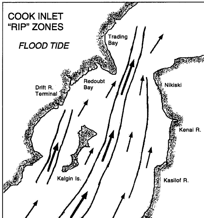
Figure 9. Cook Inlet "rip" zones – flood tide.
