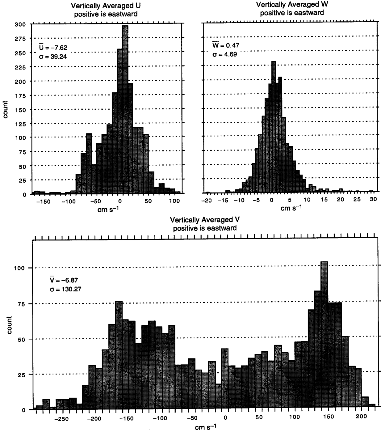
Figure 2. Cook Inlet velocity distributions.
