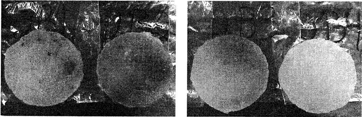
Figure 1. Large Local Variability of Sediment Concentration
