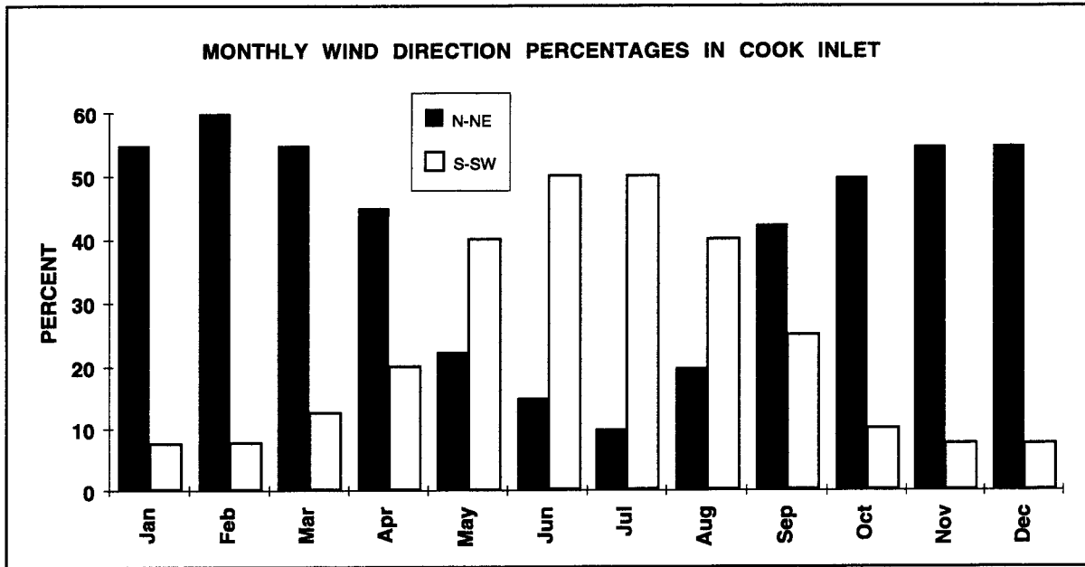
Figure 11. Monthly wind direction percentages in Cook Inlet.
