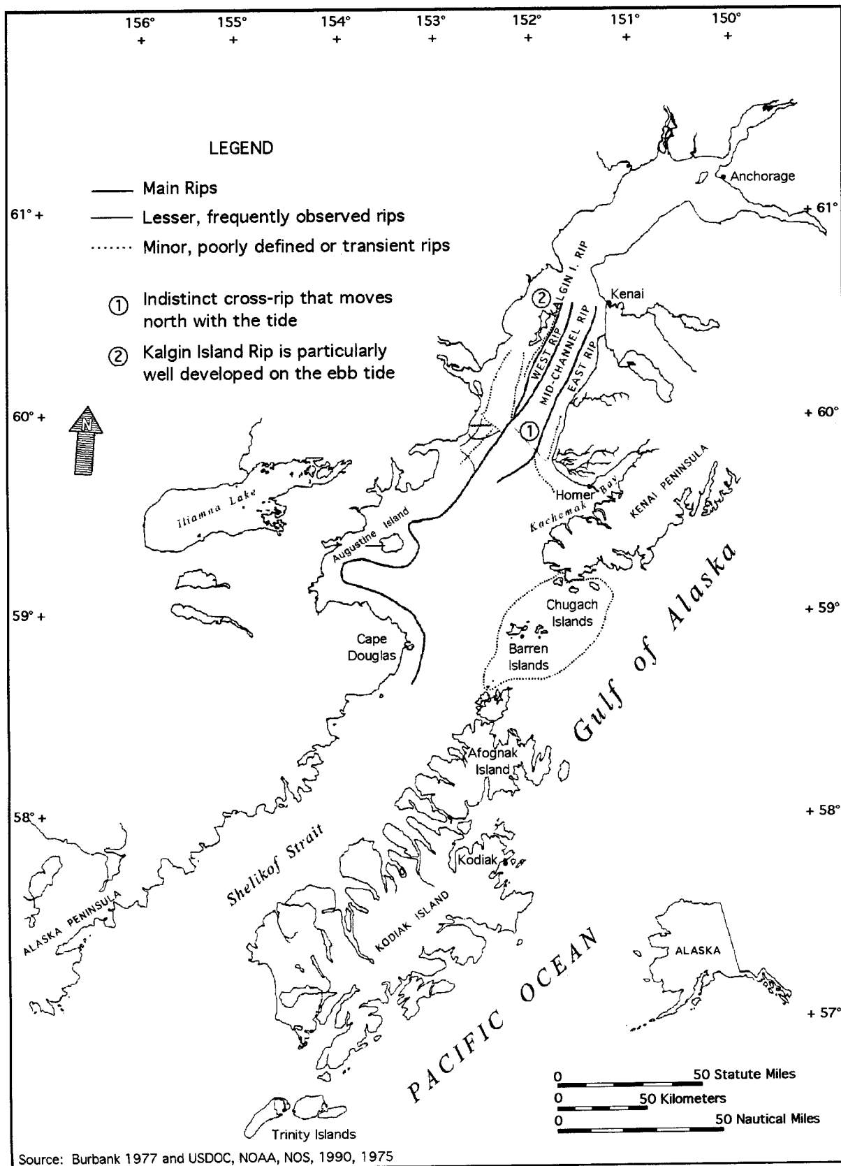
Figure 1. Historic view of rip tides in Cook Inlet.
