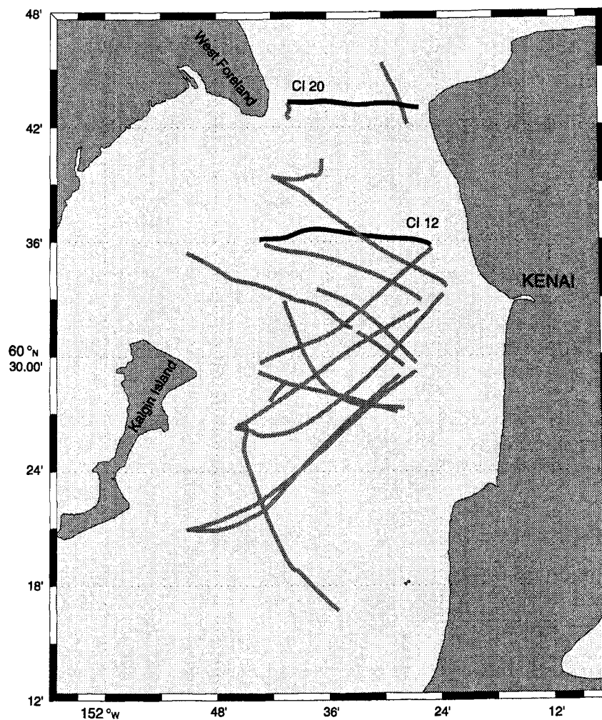
Figure 1. Acoustic Doppler current profile locations, CIRCAC Cook Inlet cruise, 16–18 June 1999.
