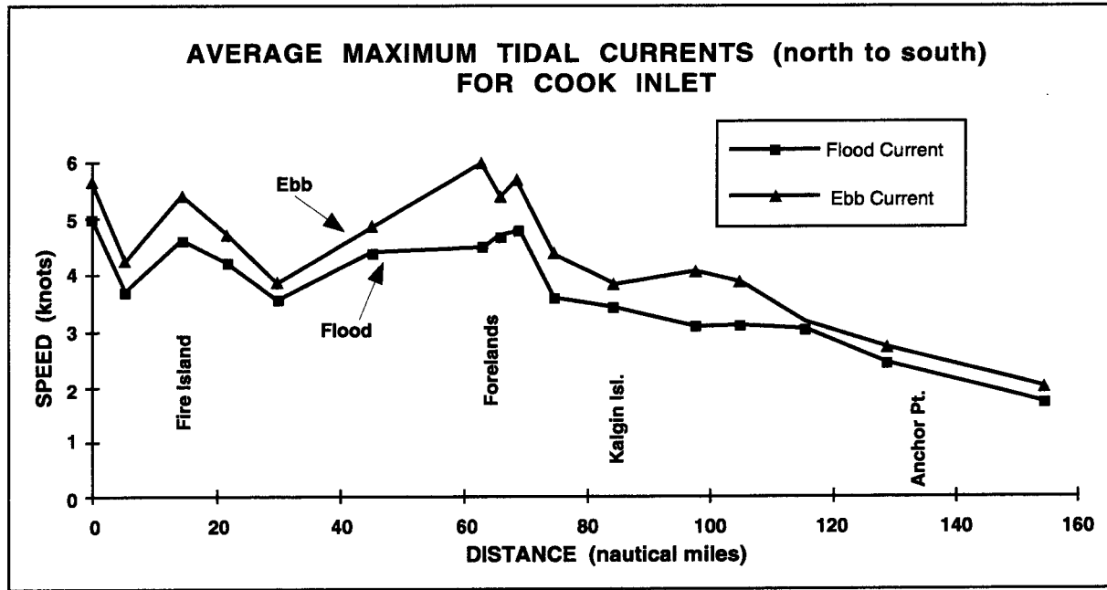
Figure 5. Average maximum tidal currents for Cook Inlet.
