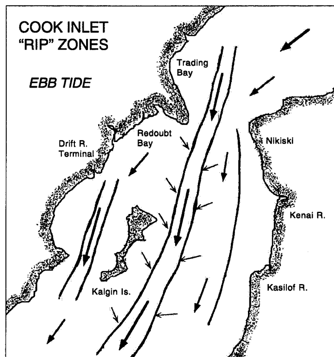
Figure 10. Cook Inlet "rip" zones – ebb tide.
