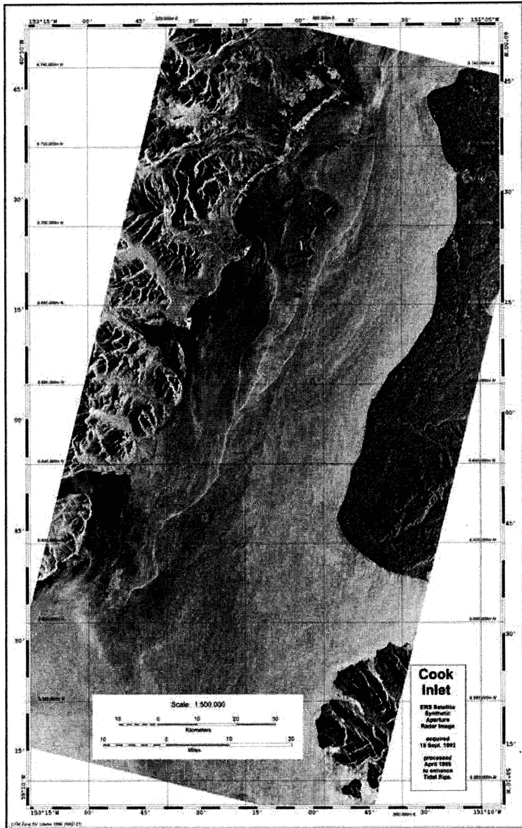
Figure 2. SAR image of Cook Inlet.
