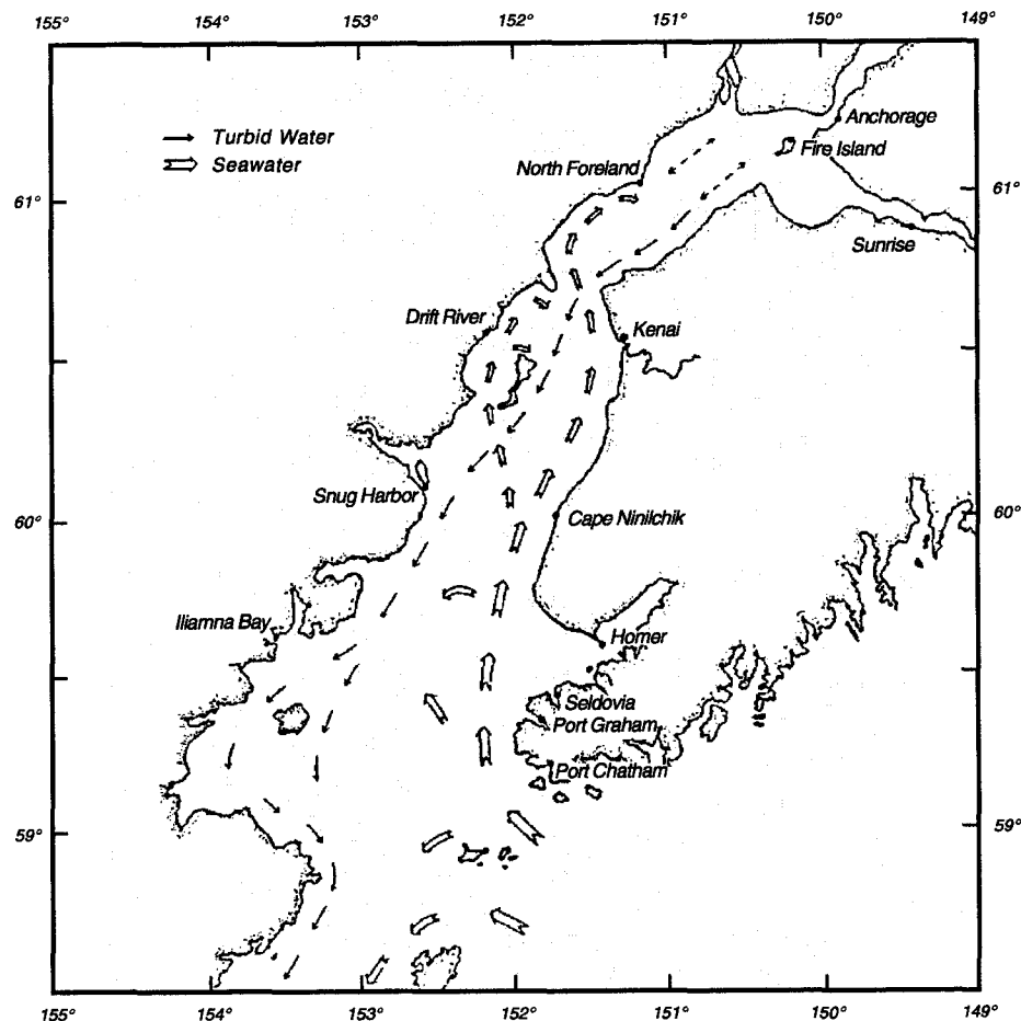
Figure 30. Net surface circulation within Cook Inlet inferred by Burbank, 1974.
