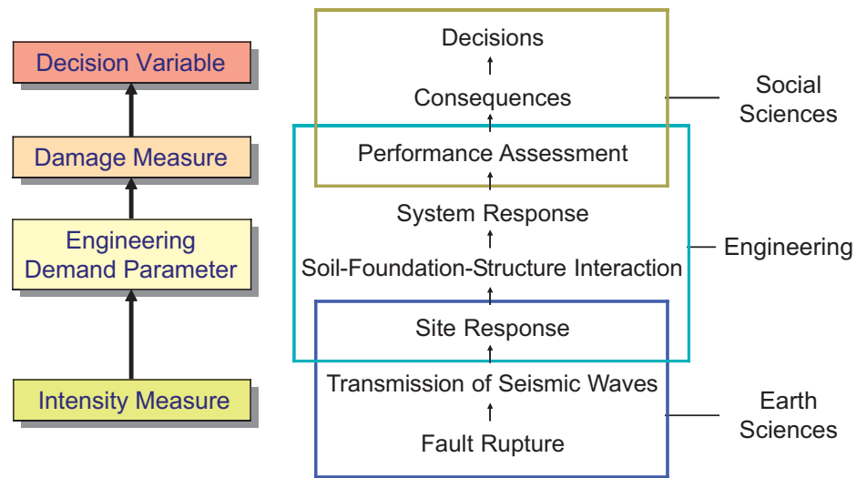
Illustration relating steps in PBEE (center) to PEER's PBEE framework variables (left) and traditional disciplines (right). Courtesy of PEER.
