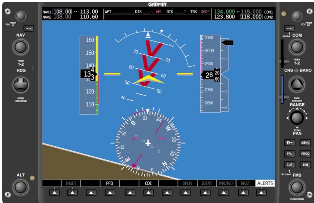
Figure 5-72. Unusual Attitude Protection With Valid AHRS.
