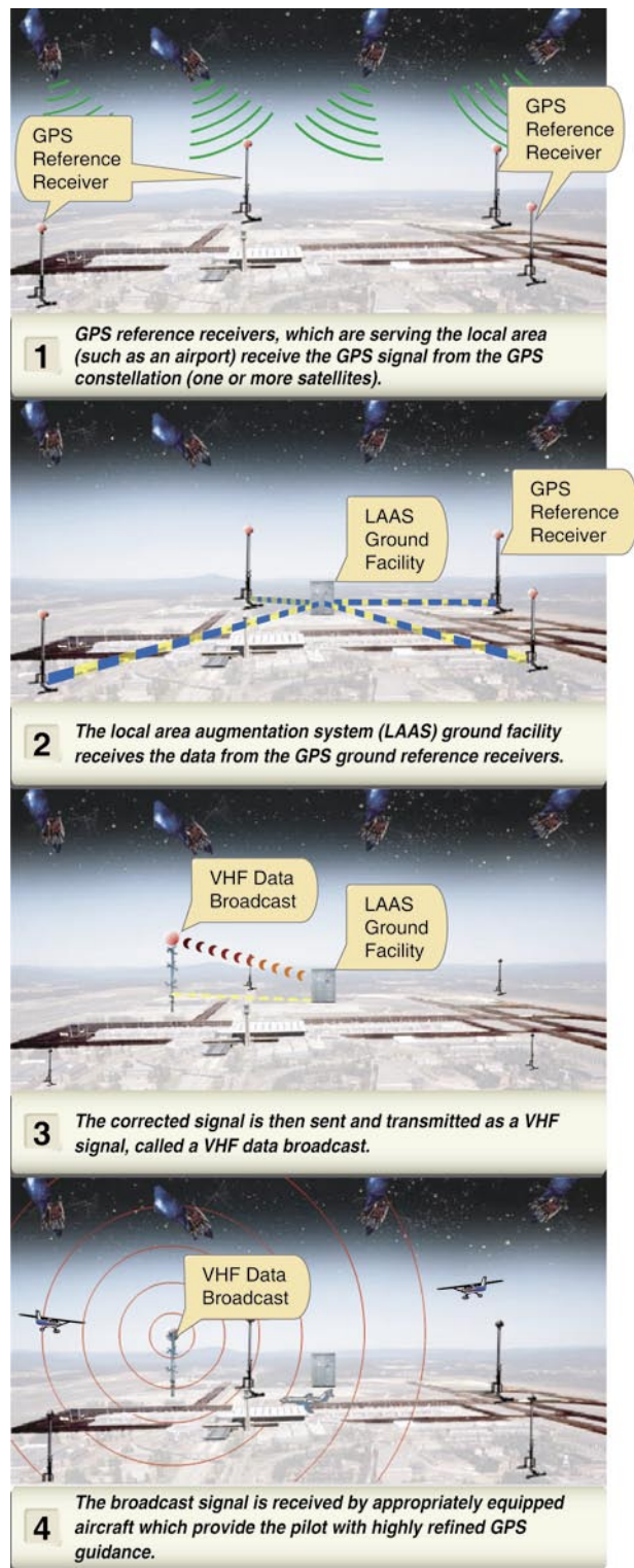
Figure 7-32. LAAS Representation.
