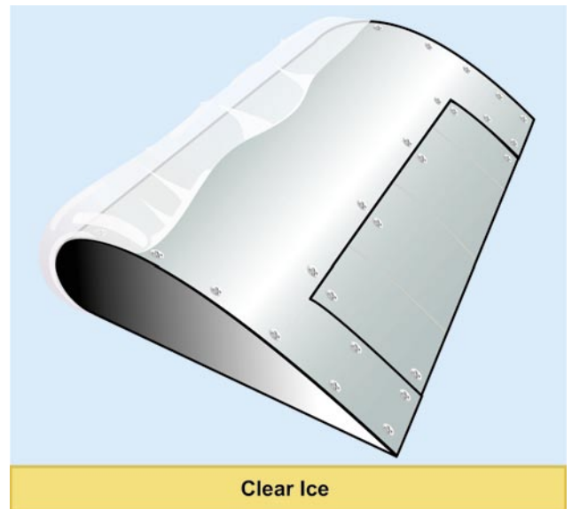
Figure 2-16. Clear Ice.
