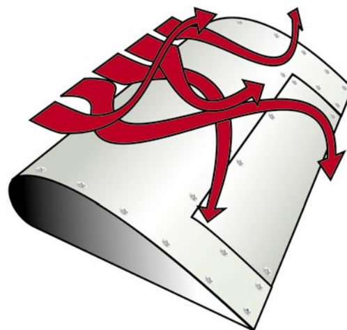
Uncontrolled Turbulence
