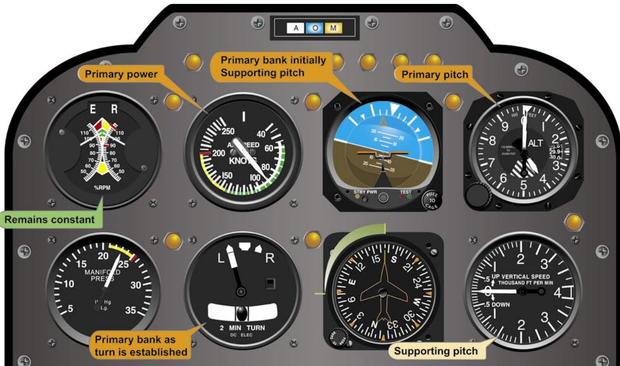
Figure 6-14. Flight Instrument Indications in a Standard-Rate Turn to the Left.
