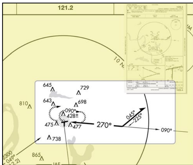
Figure 8-13. 45° Procedure Turn.
