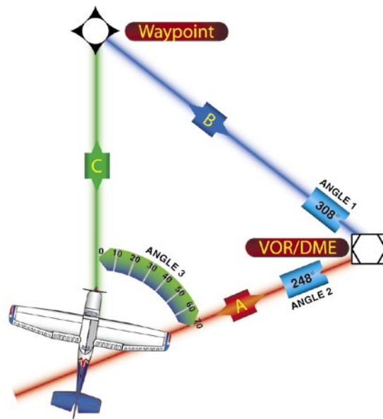
Figure 7-22. RNAV Computation.
