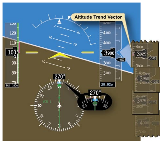
Figure 4-31. Supporting Instruments.
