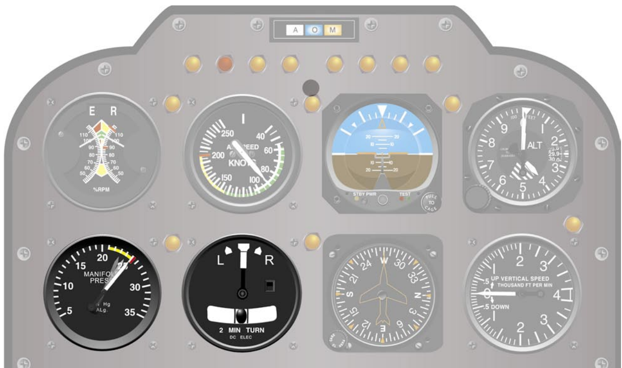
Figure 6-6. Coordinated flight is indicated by centering of the ball.
