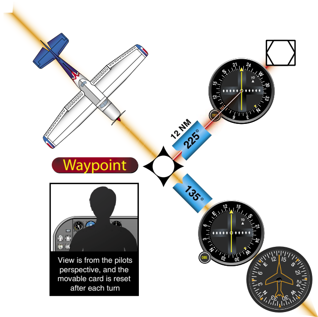
Figure 7-25. Aircraft/DME/Waypoint Relationship.
