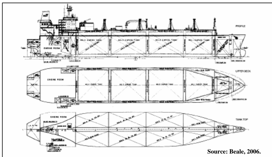
Figure 62. LNG Tanker Design with Double Membrane Tanks.
