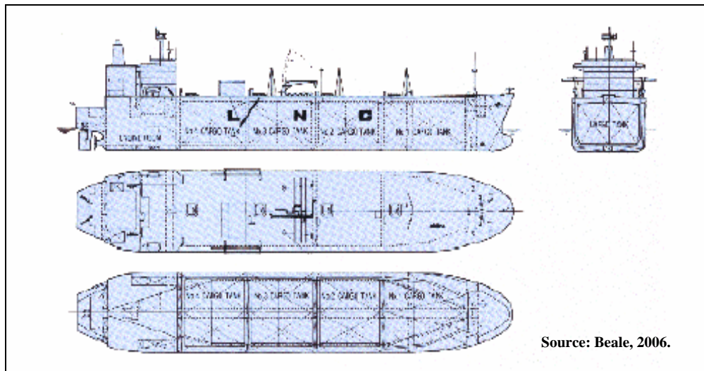
Figure 60. LNG Tanker Design with Prismatic Tanks.
