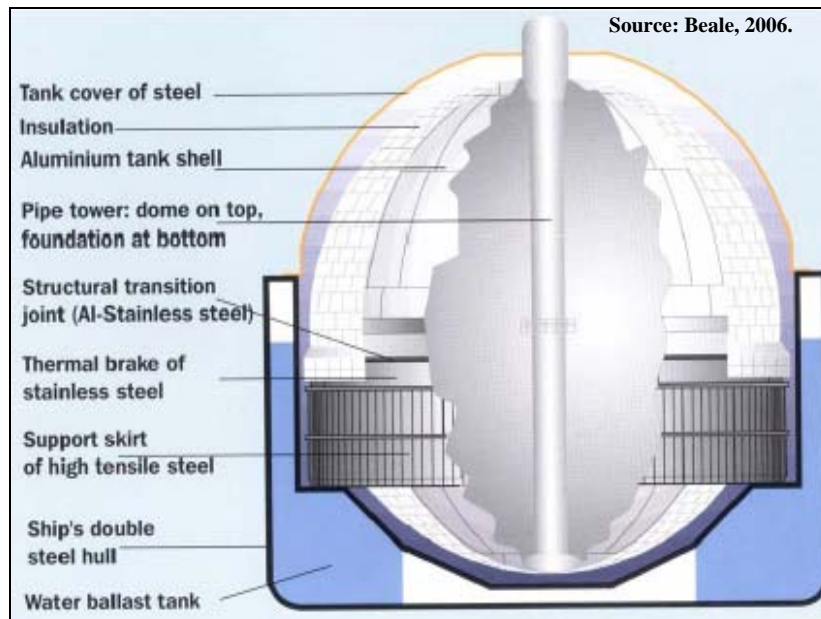
Figure 58. Spherical Tank Design.
