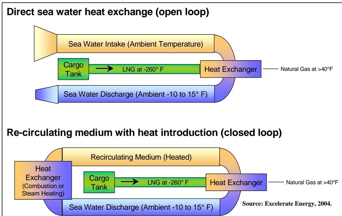
Figure 69. Primary Methods to Vaporize LNG.
