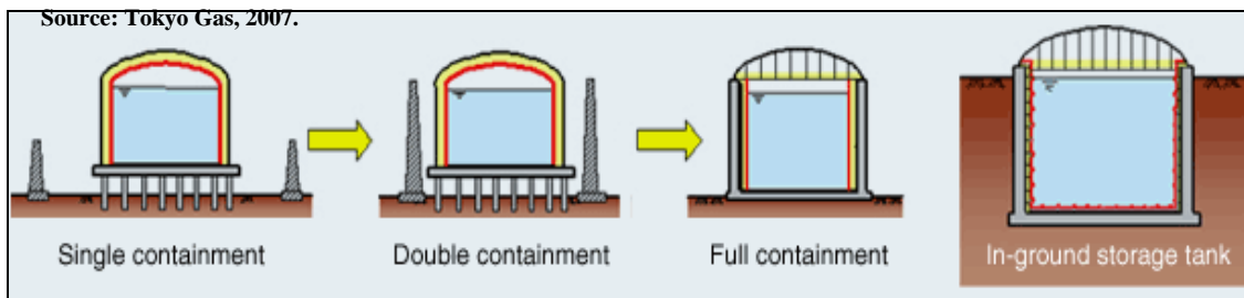
Figure 66. Types of LNG Storage Tanks.
