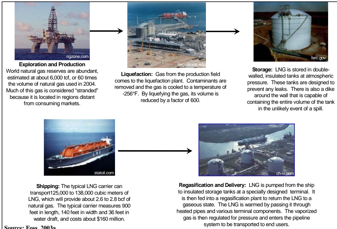
Figure 35. LNG Schematic, Production to End-User.
