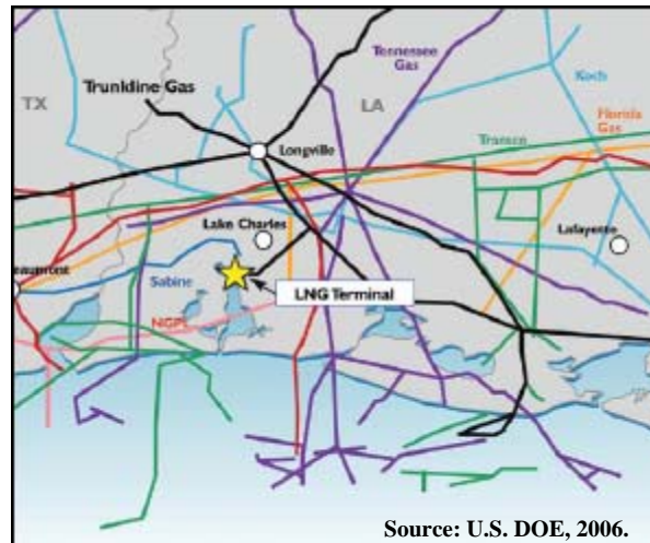
Figure 68. Lake Charles LNG Facility and Surrounding Pipelines.
