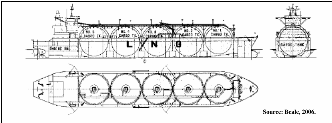
Figure 57. LNG Tanker Design with Spherical Tanks.
