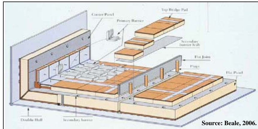
Figure 63. Membrane Tank Design.
