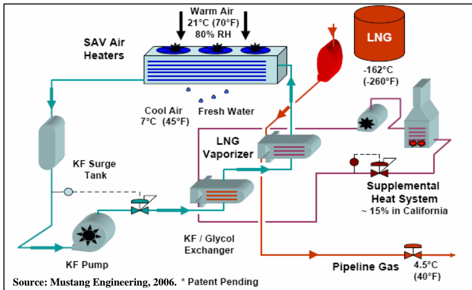
Figure 70. Mustang LNG Smart™ Ambient Air Vaporization Process.
