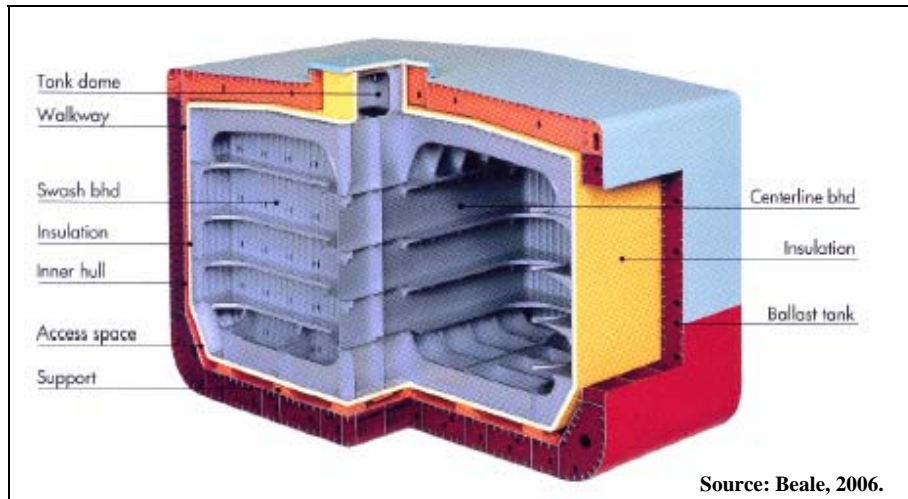
Figure 61. Prismatic Tank Design
