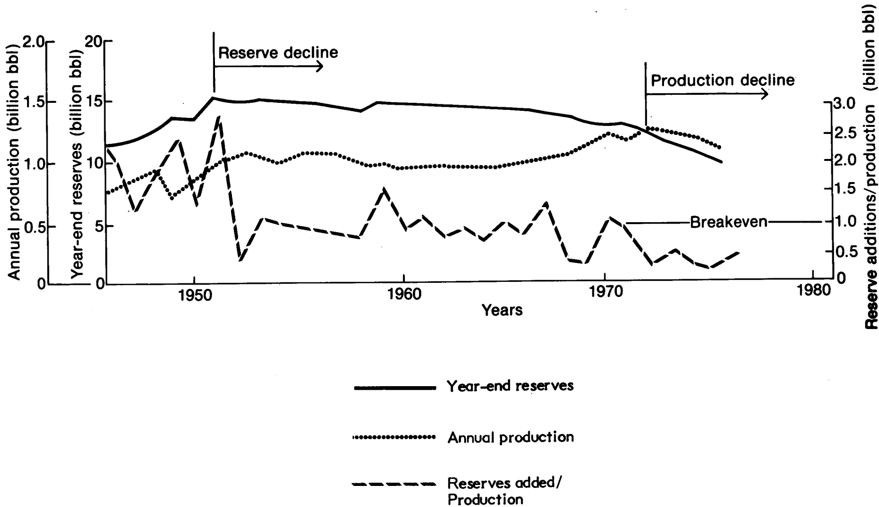
Figure OAG-1. Texas crude oil production and reserve trends (Fisher 1978).
