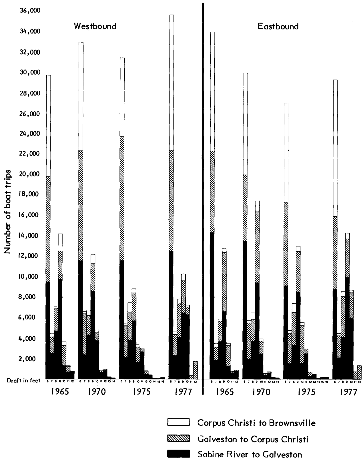
Figure TRANS-2. Distribution of Gulf Intracoastal Waterway (GIWW) boat traffic by reach, direction, and draft, for selected years 1965 through 1977 (U.S. Dept. of the Army, Corps of Engineers 1966, 1971, 1976, 1978).
