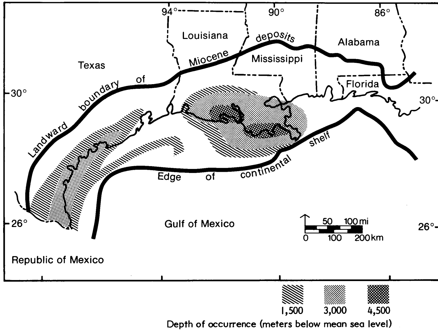
Figure OAG-4. Location and depth of occurrence of the geopressured zone in the northern Gulf of Mexico basin (Dorfman and Kehle 1974).
