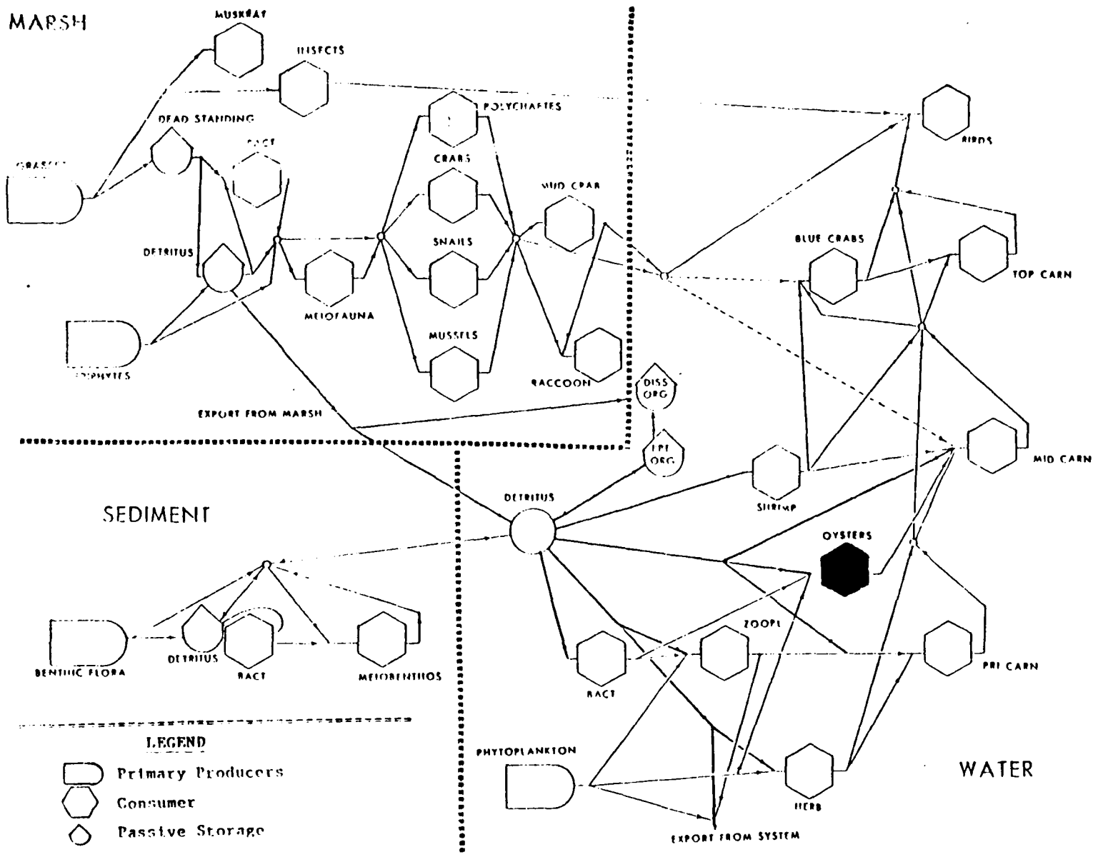
Figure 15. Diagram of marsh-estuary system showing components and pathways. Heavy lines indicate flow of detritus (adapted from Day et al. 1973).
