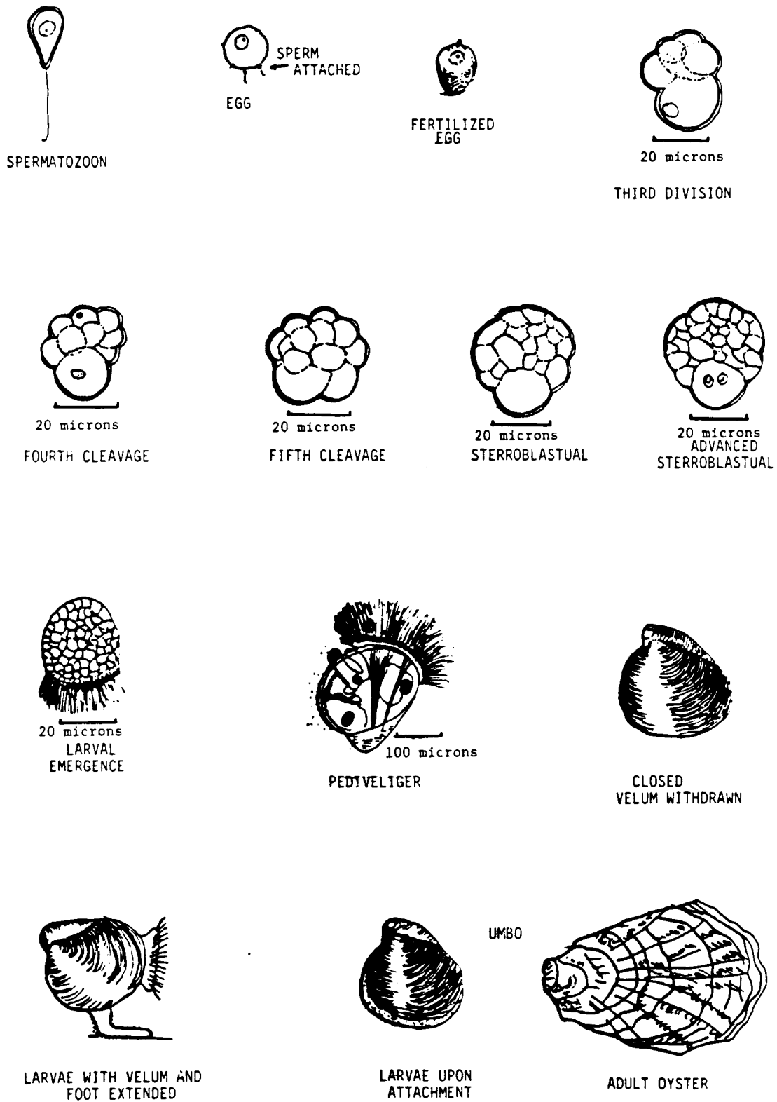
Figure 13. Larval stages of Crassostrea virginica .
