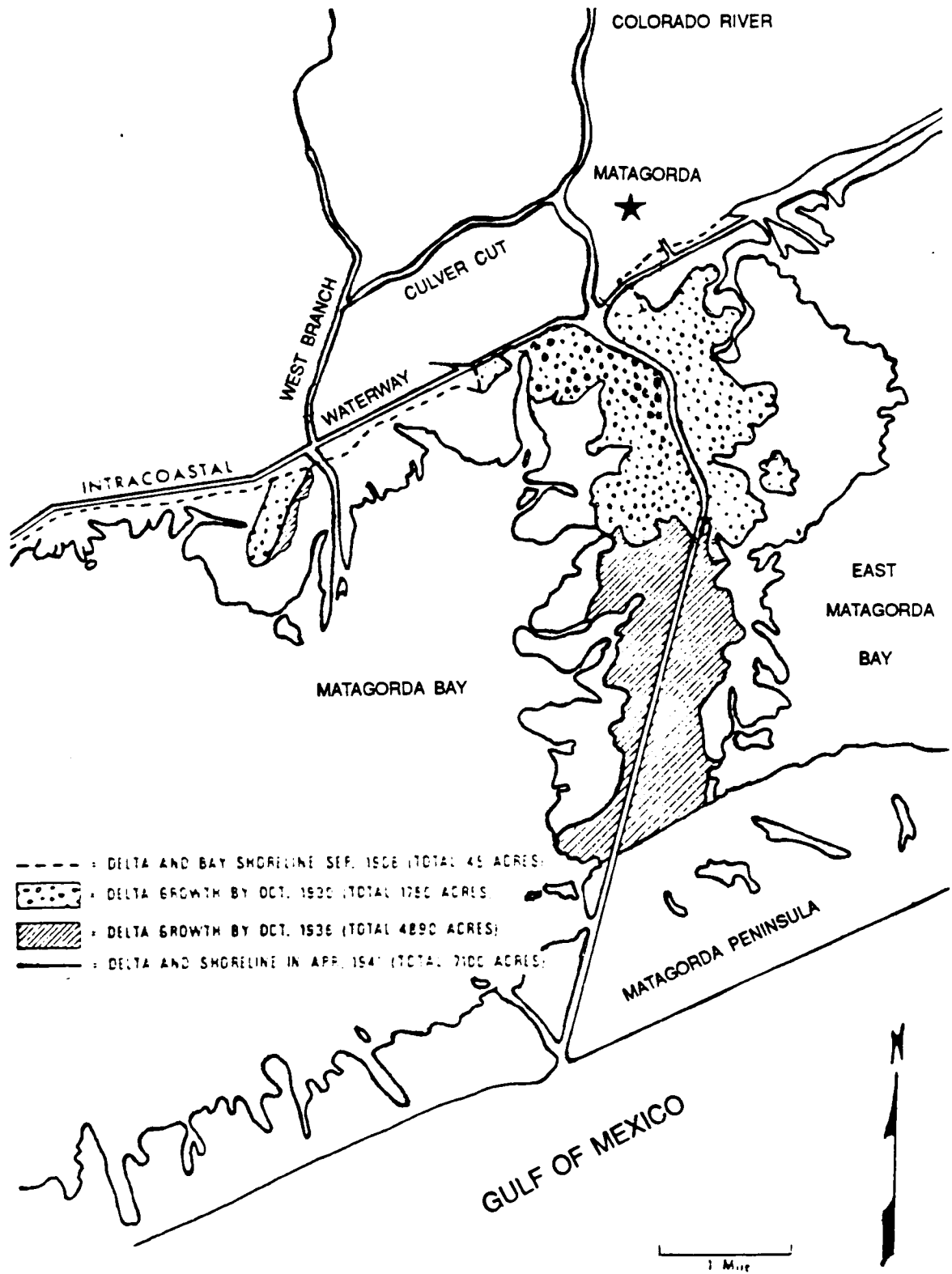
Figure 4. Successive growth stages of the modern delta of the Colorado River, September 1908 to April 1941 (after Wadsworth 1966).
