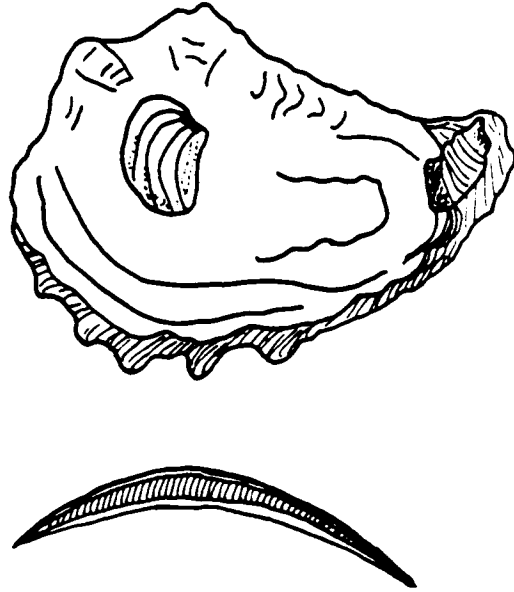
Figure 12. Shell structure of Crassostrea virginica .
