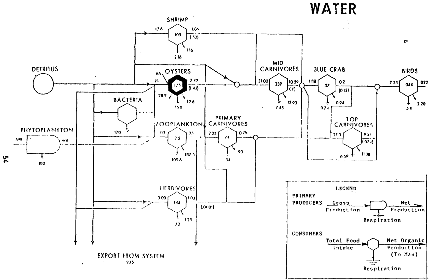
Figure 16. Summary of carbon flow in estuarine water column. Units are grams of organic matter/m 2 /yr.
