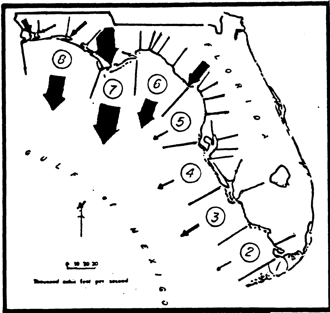
Figure 9. Relative discharge of the principal gauged streams of the Florida west coast (see Table 9) (after McNulty et al. 1972).
