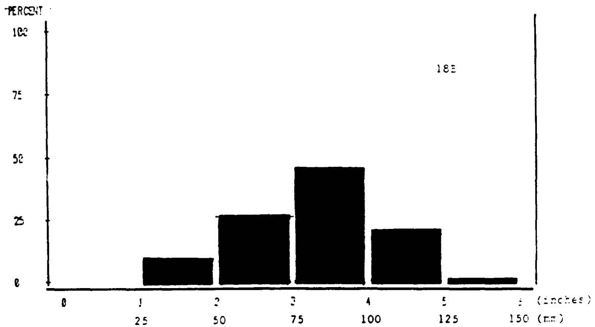
Figure 18. Size frequency distribution of oysters on reefs in Louisiana. A. Reef in an area of natural reproduction. B. Reef in an area of low natural reproduction; seed oysters planted by an oyster fisherman.
