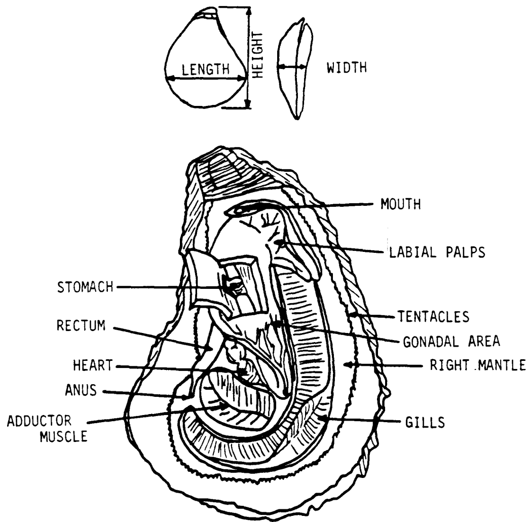
Figure 11. The general structure of Crassostrea virginica .
