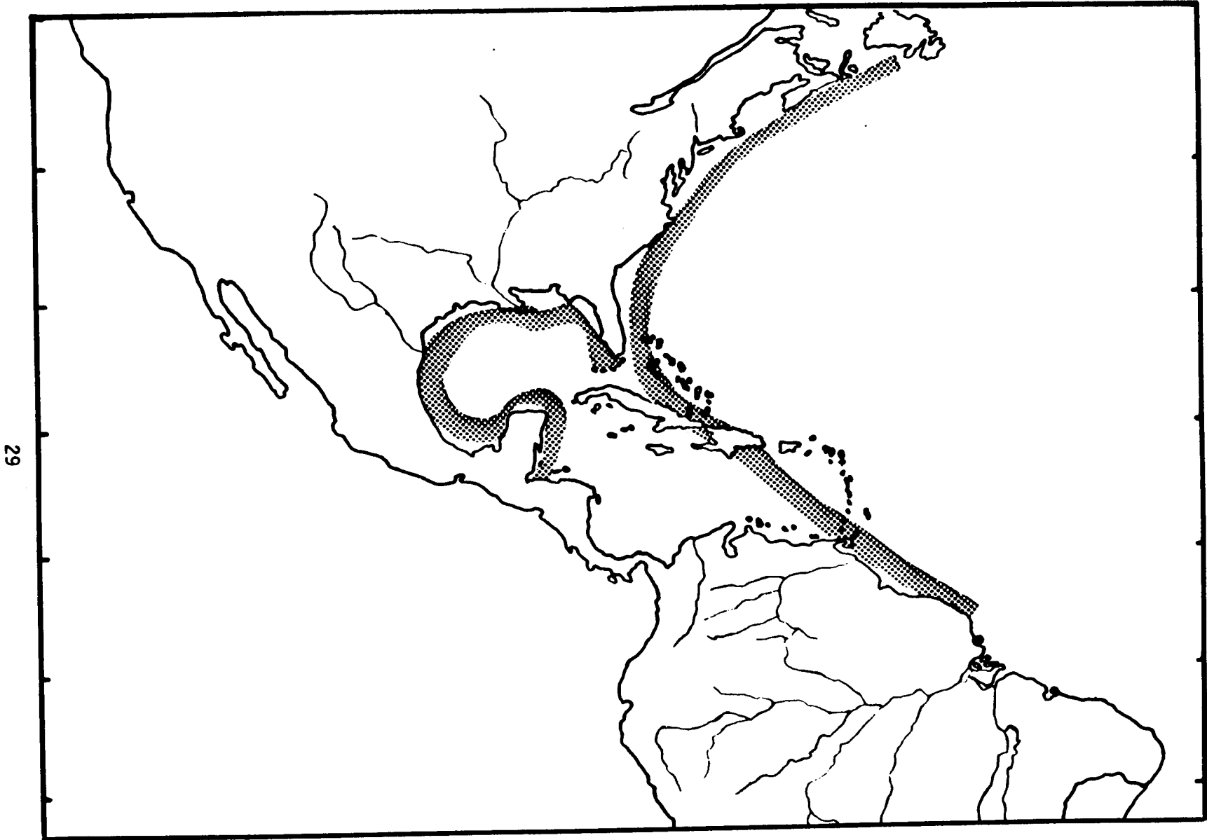
Figure 10. The distribution of Crassostrea virginica within the Americas (adapted from Ahmed 1975).
