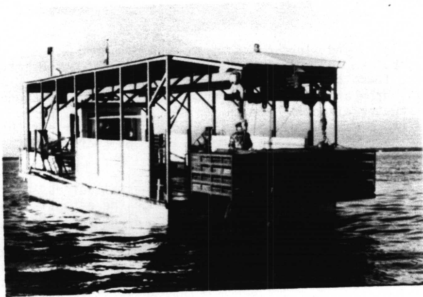
Figure 22. Containerized relaying as practiced in Mississippi.
