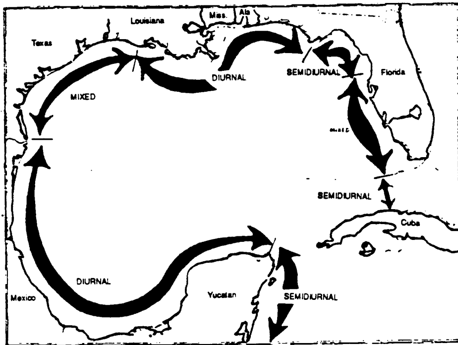
Figure 2. Gulf of Mexico tidal regimes (after Eleuterius 1975).
