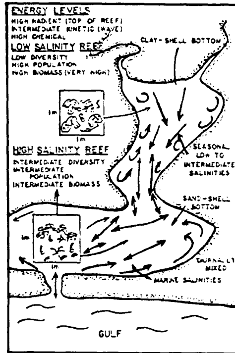
Figure 14. Diagrammatic representation of the mollusk (oyster or mussel) or serpulid reef ecosystem with typical environmental and faunal characteristics. (Adapted from Parker 1975).
