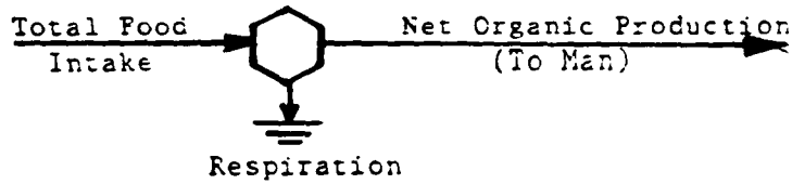
Figure 17. Energy flow of oyster biomass in estuarine system, in grams of organic matter/m 2 /yr (adapted from Day et al. 1973).
