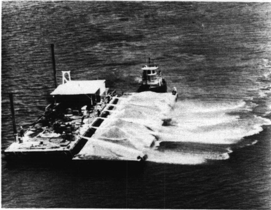
Figure 23. Shell planting operation in Louisiana.
