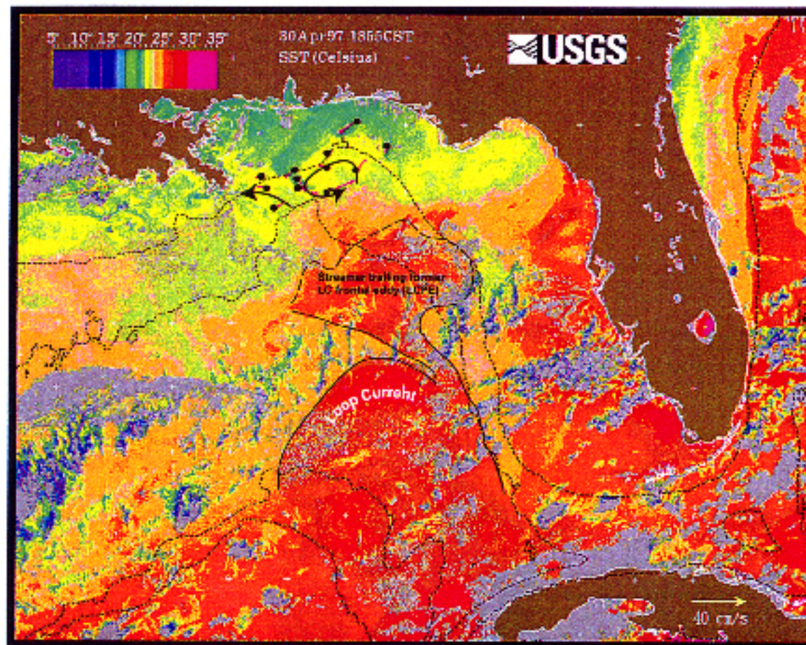
Figure 4.2-3. SST image for April 30, 1997 (1355 CST). Measured surface current vectors are overlaid on the image in the study area. A streamer trailing a former LC frontal eddy is labelled, as is the Loop Current proper.
