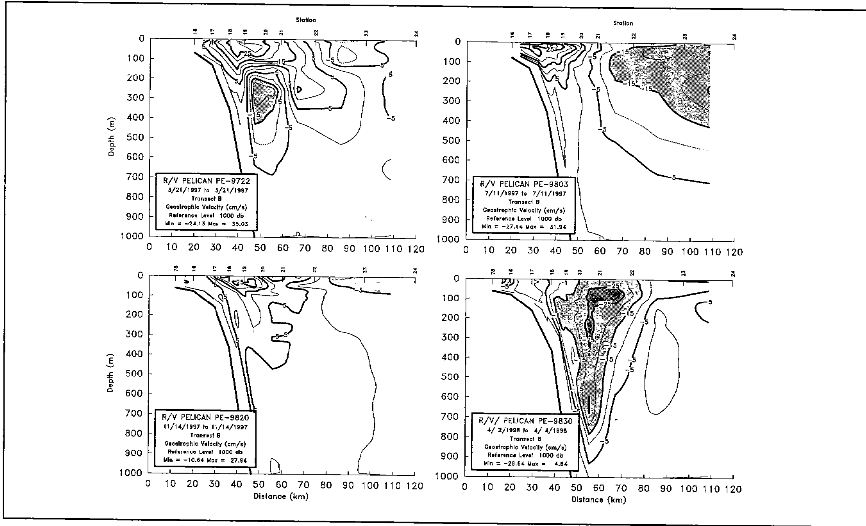
Figure 4.2-8. Geostrophic velocities on Section B for the indicated surveys. Positive velocities are eastward, normal to the section. Higher westward (negative) velocities are shaded.
