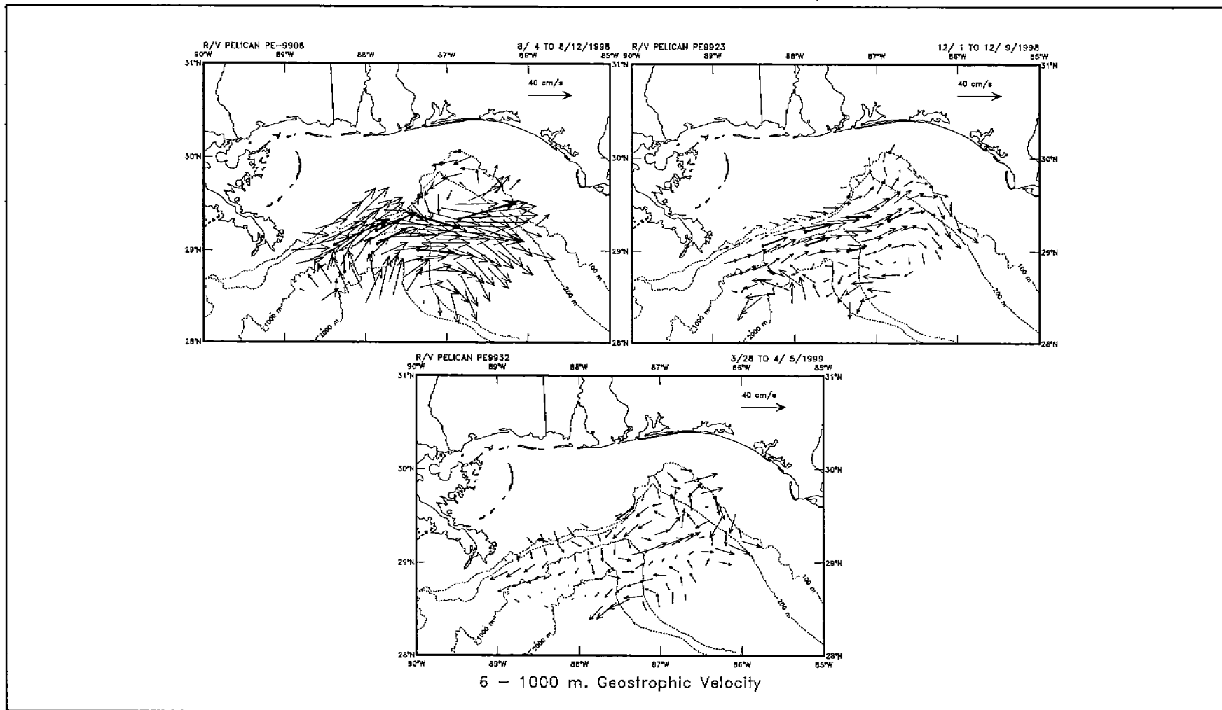
Figure 4.2-7. Geostrophic velocities at 6m from the hydrographic surveys. 5-day average velocity vectors (heavy arrows) from the 8m depth of the ADCP's are shown at stations marked with a dot.
