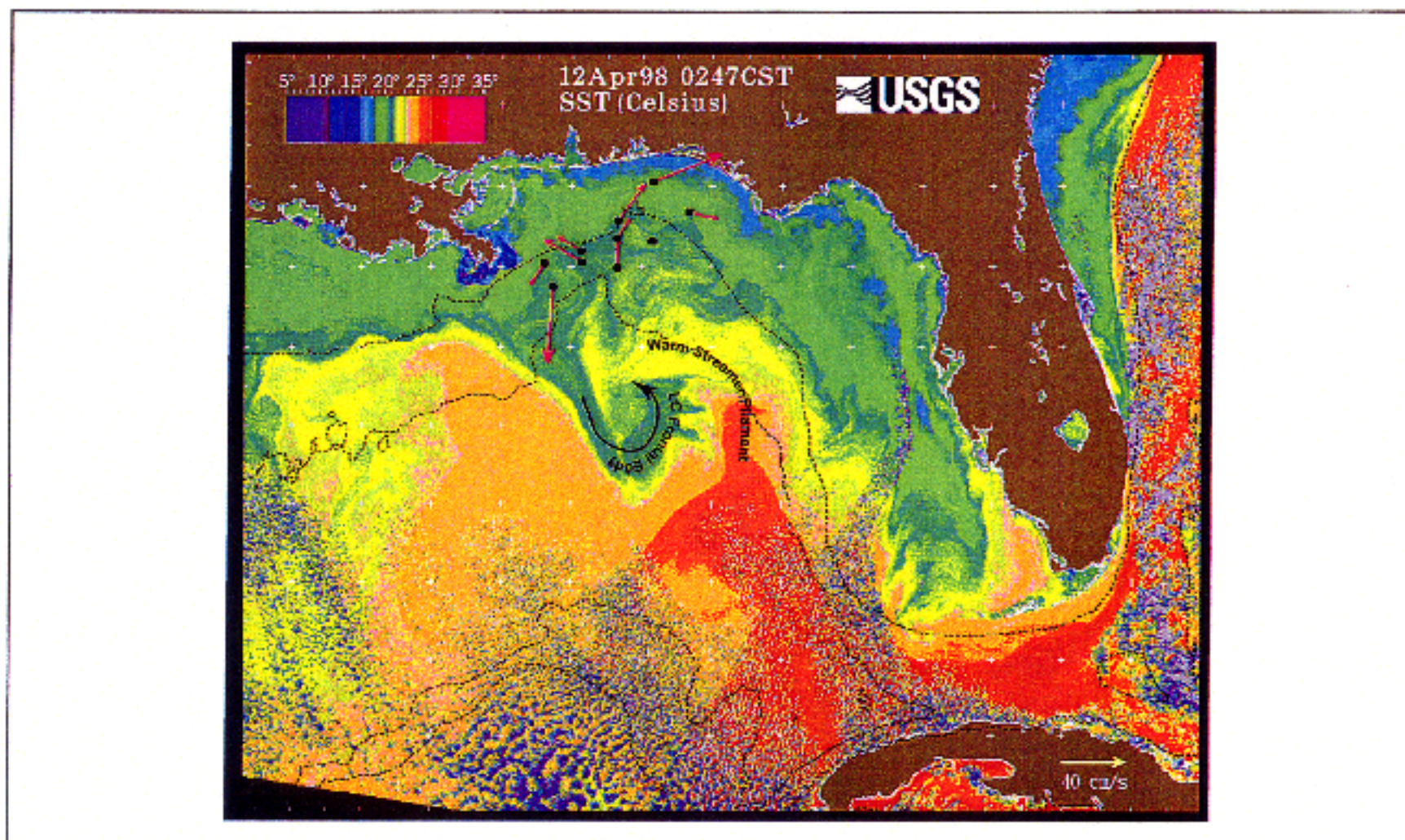
Figure 4.2-1. SST image for April 12, 1998 (0247 CST). Measured current vectors are overlaid on the image in the study area. Features mentioned in the text have been labelled for clarity.
