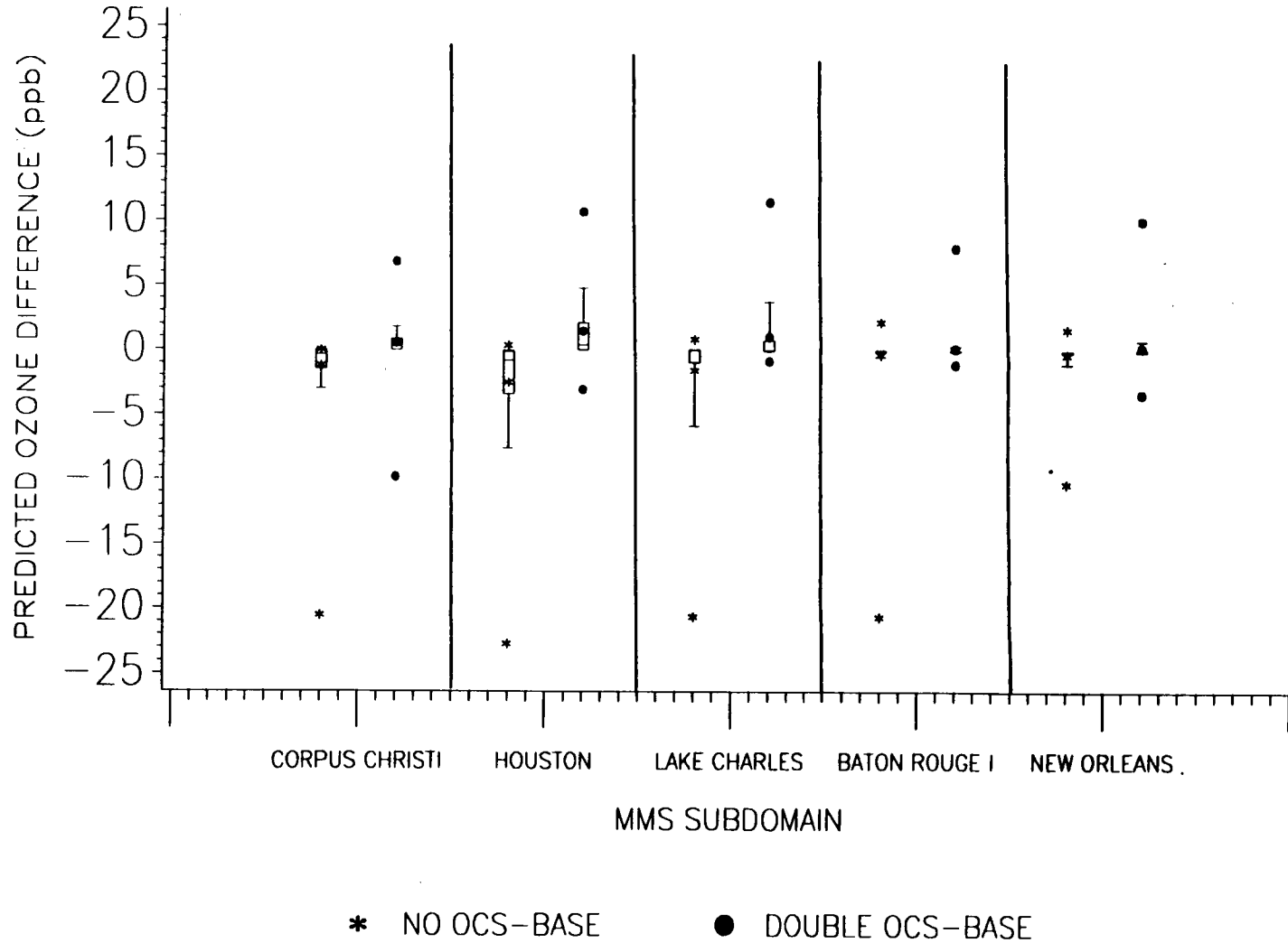
Figure 6-9. BOX PLOT OF OCS IMPACT ON MMS SUBREGIONS EPISODE #2: JULY 26 – JULY 31, 1990 (8 a.m. – 7 p.m.)
