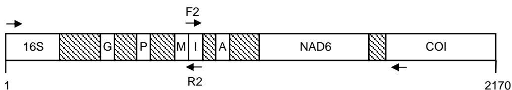
Figure 1. Inferred gene structure of a portion of mtDNA from Bugula neritina . Specific primers were designed to the 16S and COI genes (indicated by arrows) and then the intervening region was amplified using PCR from both a ‘shallow’ and a ‘deep’ type individual based on their COI sequence. The PCR product was approximately 1550 bp in length and sequencing followed by BLAST searches identified that it contained the NAD6 gene. We also identified tRNA genes for glycine (G), proline (P), methionine (M), isoleucine (I) and arginine (A). Shaded boxed indicate non-coding sequences. Total length in base pairs is noted.
