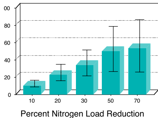
Figure 2. Forecasts from the NECOP water quality model for changes in bottom water dissolved oxygen concentration in response to nitrogen load reductions from the Mississippi River Basin.
