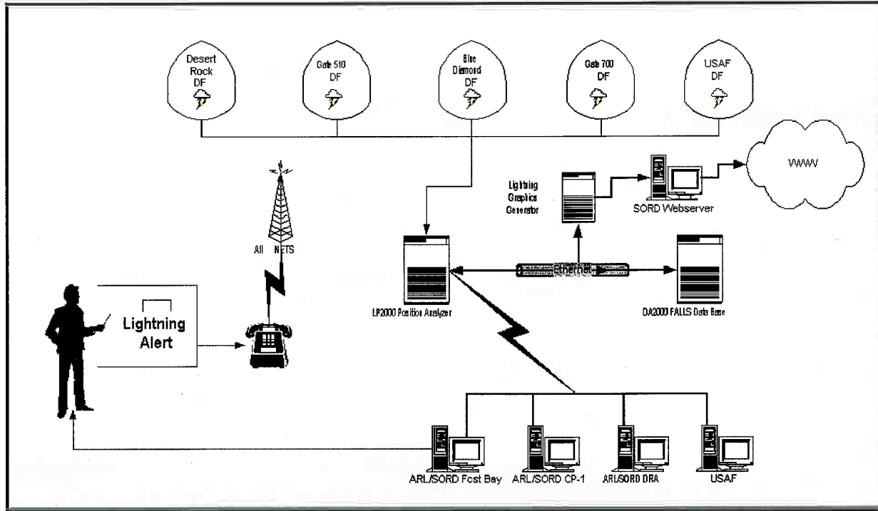
Figure 1 NTS Lightning data distribution and alert system.
