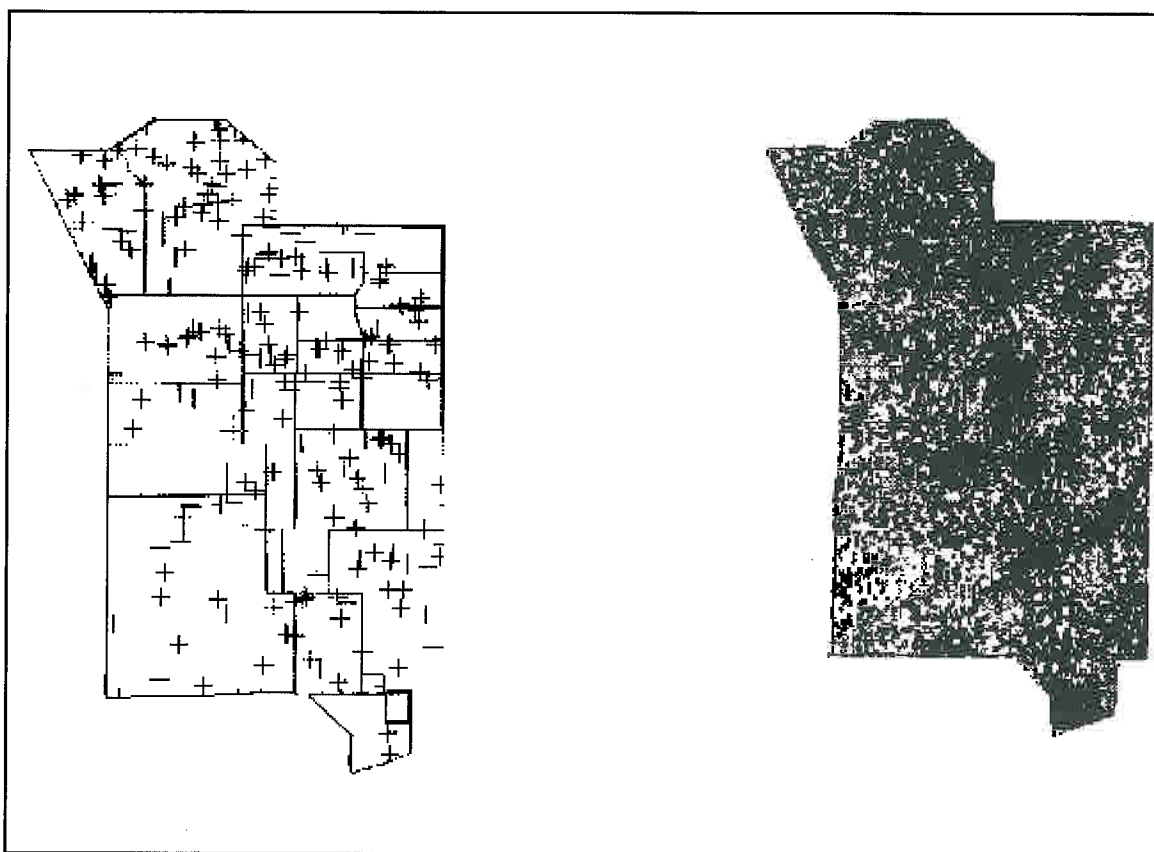
Figure 6. Distribution of warm-season positive CG flashes for 1993 through 2000 for the NTS.
