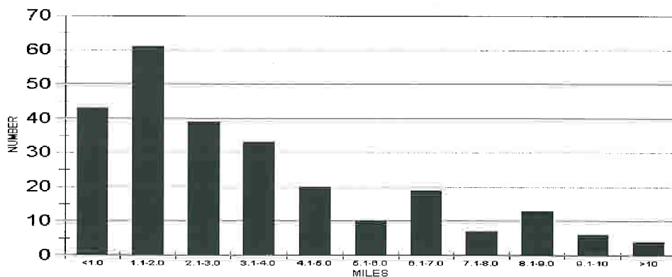
Figure 10. Distance between successive warm-season CG flashes on the NTS.
