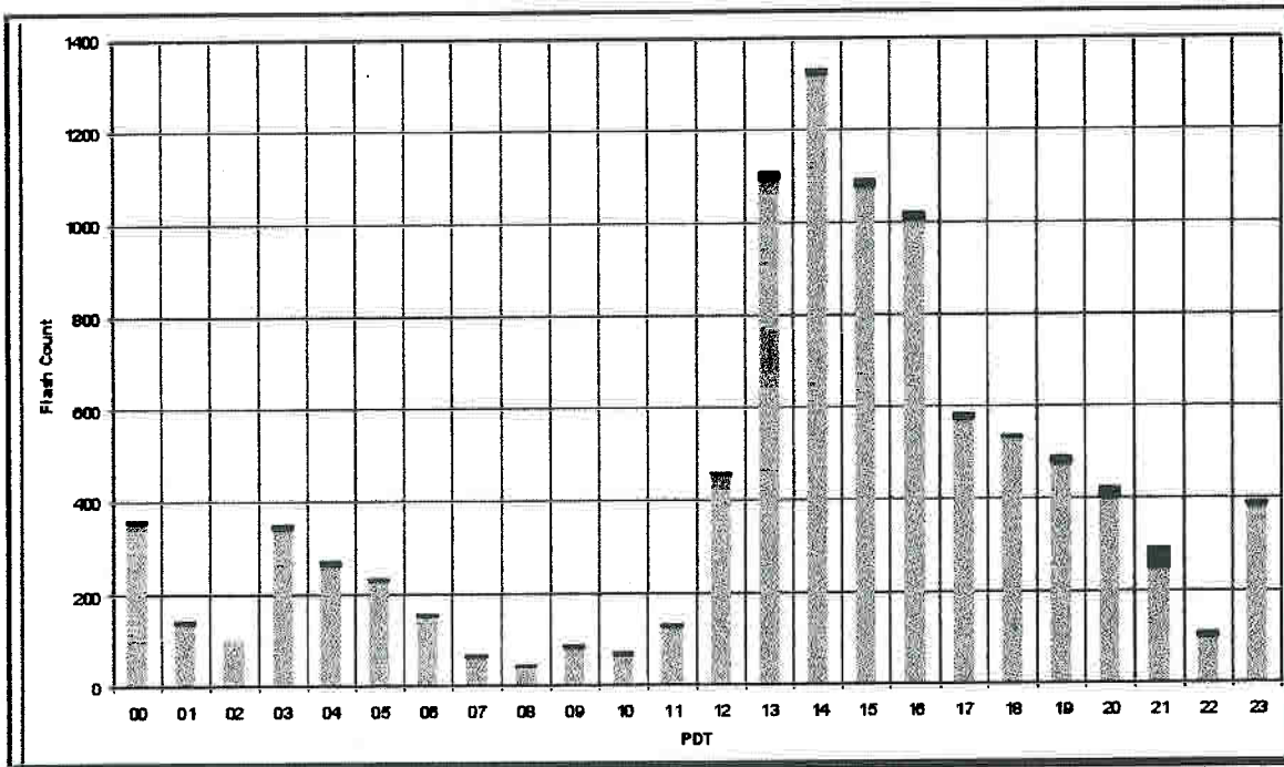
Figure 9. Diurnal distribution of CG flashes on the NTS for the warm seasons, 1993 through 2000. Time is in Pacific Daylight Time. Negative flashes are represented by the gray bars and the positive flashes by the black bars.
