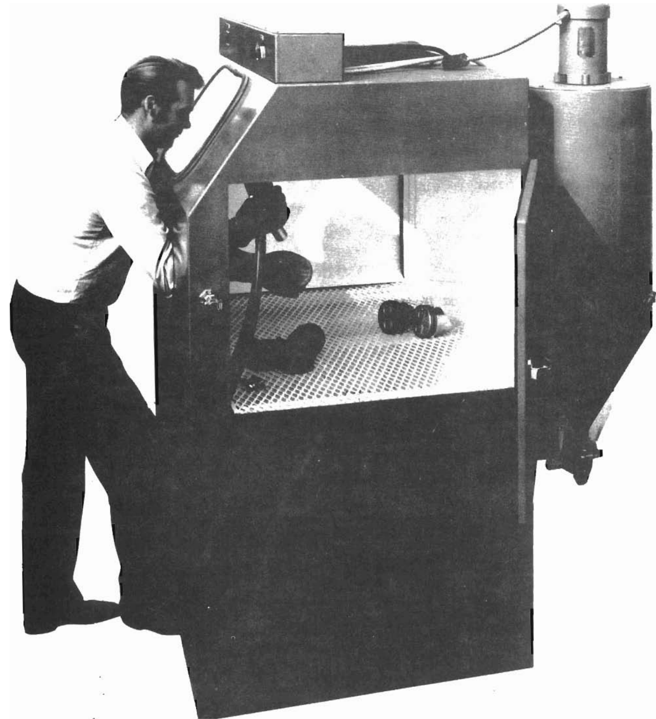
FIGURE II-7 Hand-operated Cabinet Type Blast Cleaning Machine
