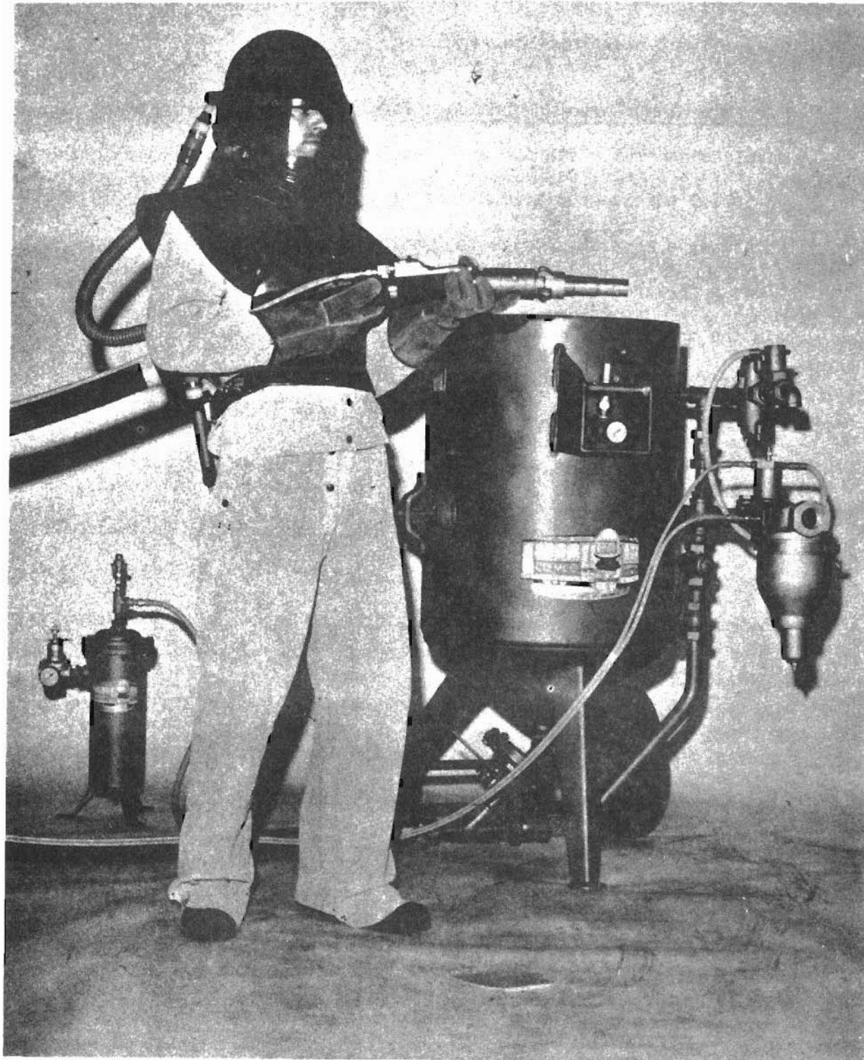
FIGURE 11-5 Portable Blast Cleaning Unit with Operator
