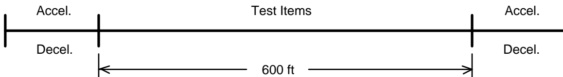
Linear Track - acceleration and deceleration length is 150 ft each end for 15 mph test speed and 0.05 g acceleration and deceleration.
