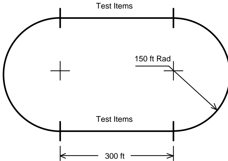
Oval Track - curved length = 942 ft
