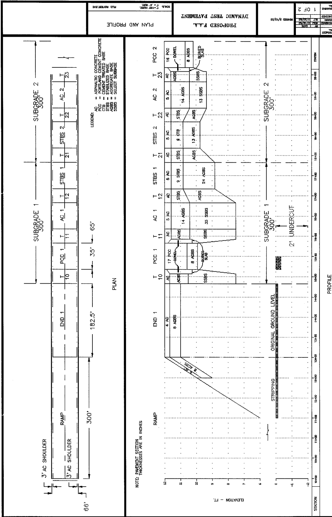
FIGURE 5-1. PLAN AND PROFILE OF TEST PAVEMENT SECTIONS
