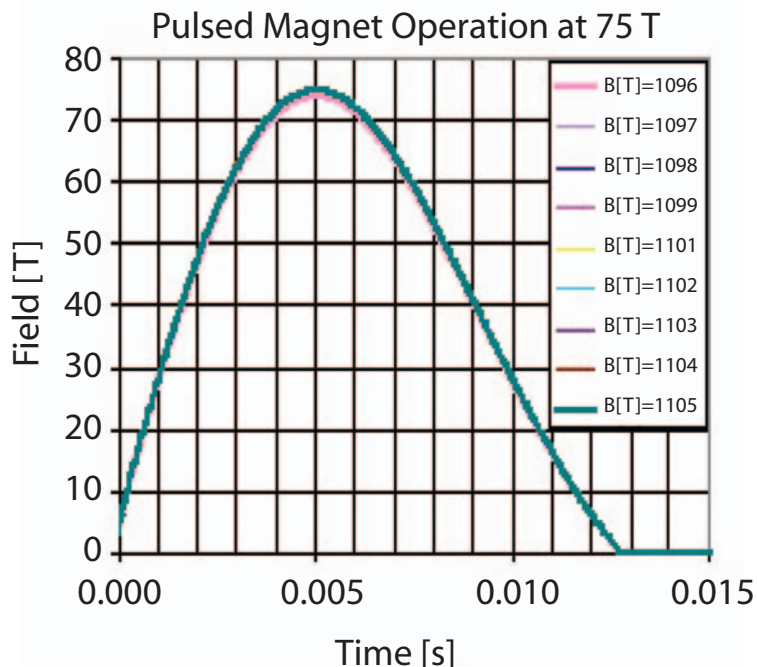
Figure 2. Pulsed field waveforms integrated from B-Dot signal.
