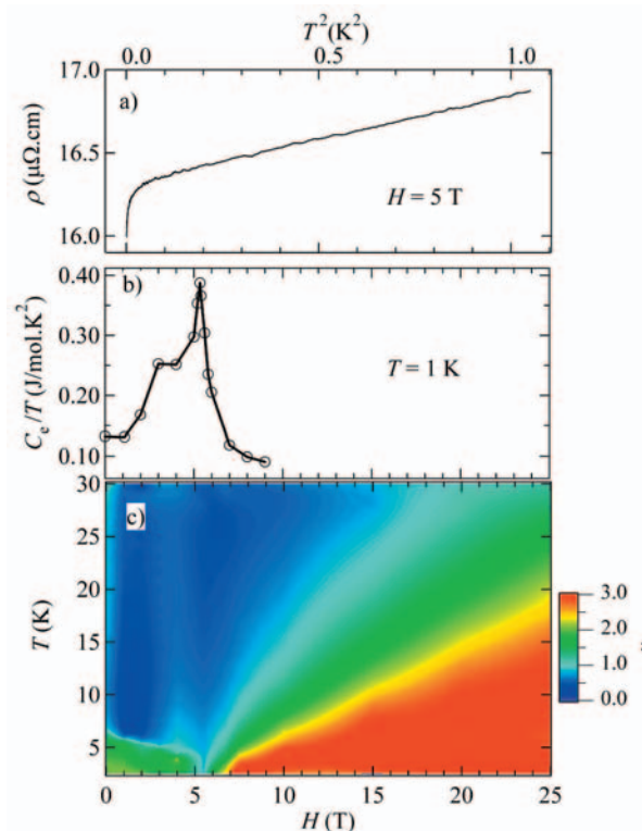
Figure 1. (a) The T^2 -dependence of \rho down to T \cong 25 mK for H = 5 \text{ T} \leq H_C . Notice the pronounced deviation from the T^2 dependence at the lowest T , which is observed only in the vicinity of the critical field H_C . (b) The electronic heat capacity as a function of field H and at T = 1 K. (c) The exponent n of the resistivity \rho in the T - H plane.
