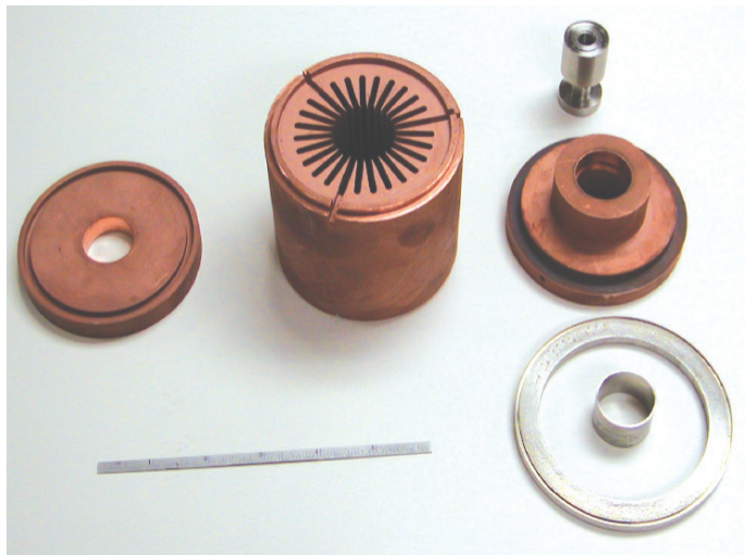
Figure 3. Heat-intercept with integral LN 2 reservoir.
