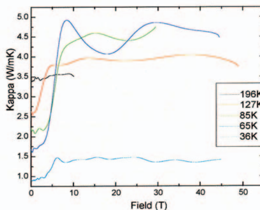
Figure 12. The 3- \omega technique was successfully tested on Nd 0.5 Sr 0.5 MnO 3 in the mid-pulse magnet.
