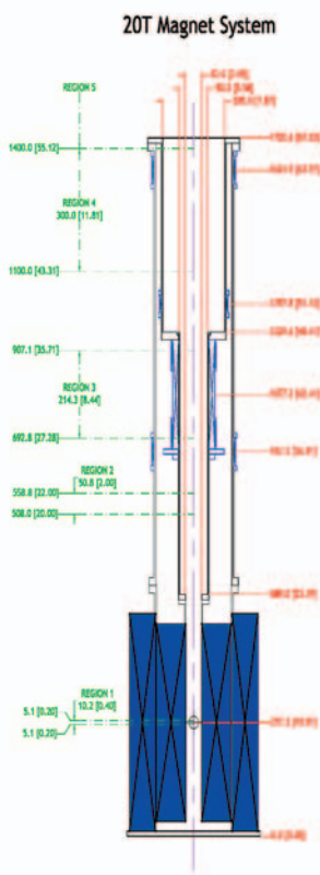
Figure 18. New 20+ T magnet system for the High B/T Facility.
