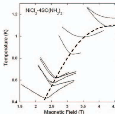
Figure 14. Adiabatic temperature sweeps as a function of magnetic field of single crystalline \text{NiCl}_2\text{-4SC(NH}_2\text{)}_2 oriented with the magnetic field parallel to the tetragonal c-axis. Dashed lines indicate the estimated onset of field-induced long-range order.
