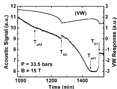
Figure 19. A_1 and A_2 transitions in superfluid ^3\text{He} at 15 T. The lower trace is the ultrasound signal, which shows the transitions of the superfluid ^3\text{He} confined in aerogel, as well as the transitions of the bulk liquid. The upper trace (marked VW) shows the bulk transitions observed simultaneously by a vibrating-wire viscometer.
