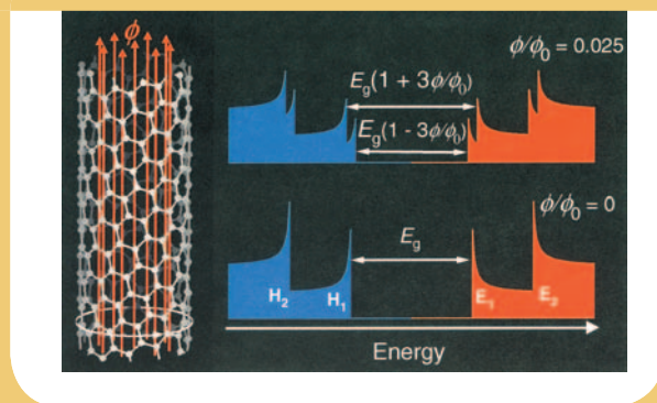
Figure 1. Schematic diagram showing band structure modifications induced by a magnetic flux threading a single-walled carbon nanotube.
