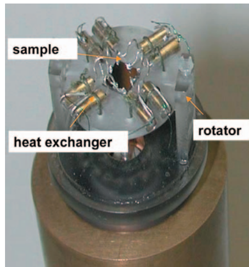
Figure 20. Ultra-low temperature sample rotator for use inside a sample chamber that is filled with liquid ^3\text{He} to keep the sample cold.
