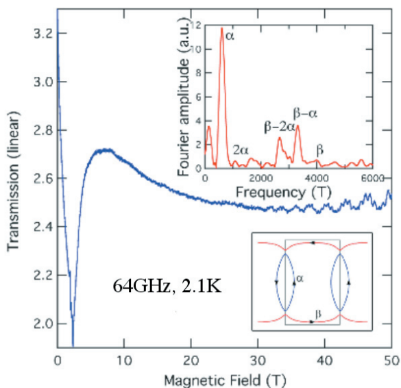
Figure 9. GHz-frequency conductivity measurements of \kappa -(BEDT-TTF) 2 Cu(SCN) 2 .
