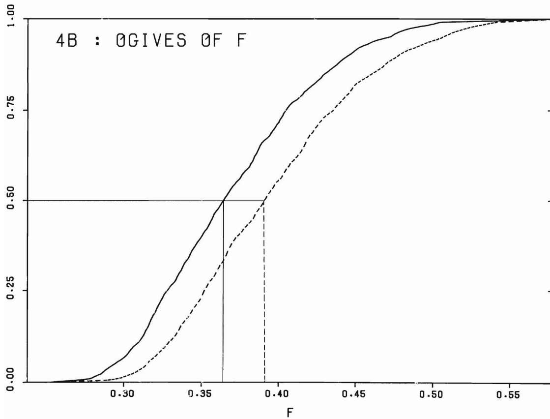
Figure 4—Probability distributions for population dynamics model parameters (a) R ; (b) F ; (c) S_0 and (d) \lambda represented by ogives. The initial distributions are shown by dashed lines; the refined distributions (incorporating the equation (15) constraint) are shown by solid lines.
