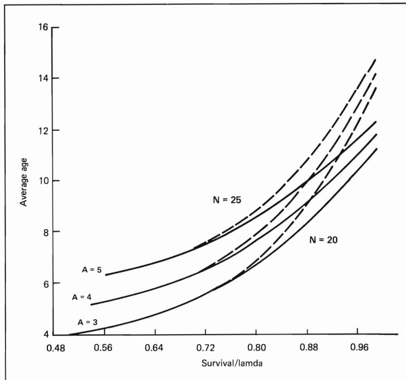
Figure 3—Average age of reproducing females as a function of the ratio of adult survival to \lambda (the exponential of the rate of increase of the population) for age at first reproduction ( a ) 3, 4, and 5, and the maximum age of reproducing females ( N ) 20 and 25.
