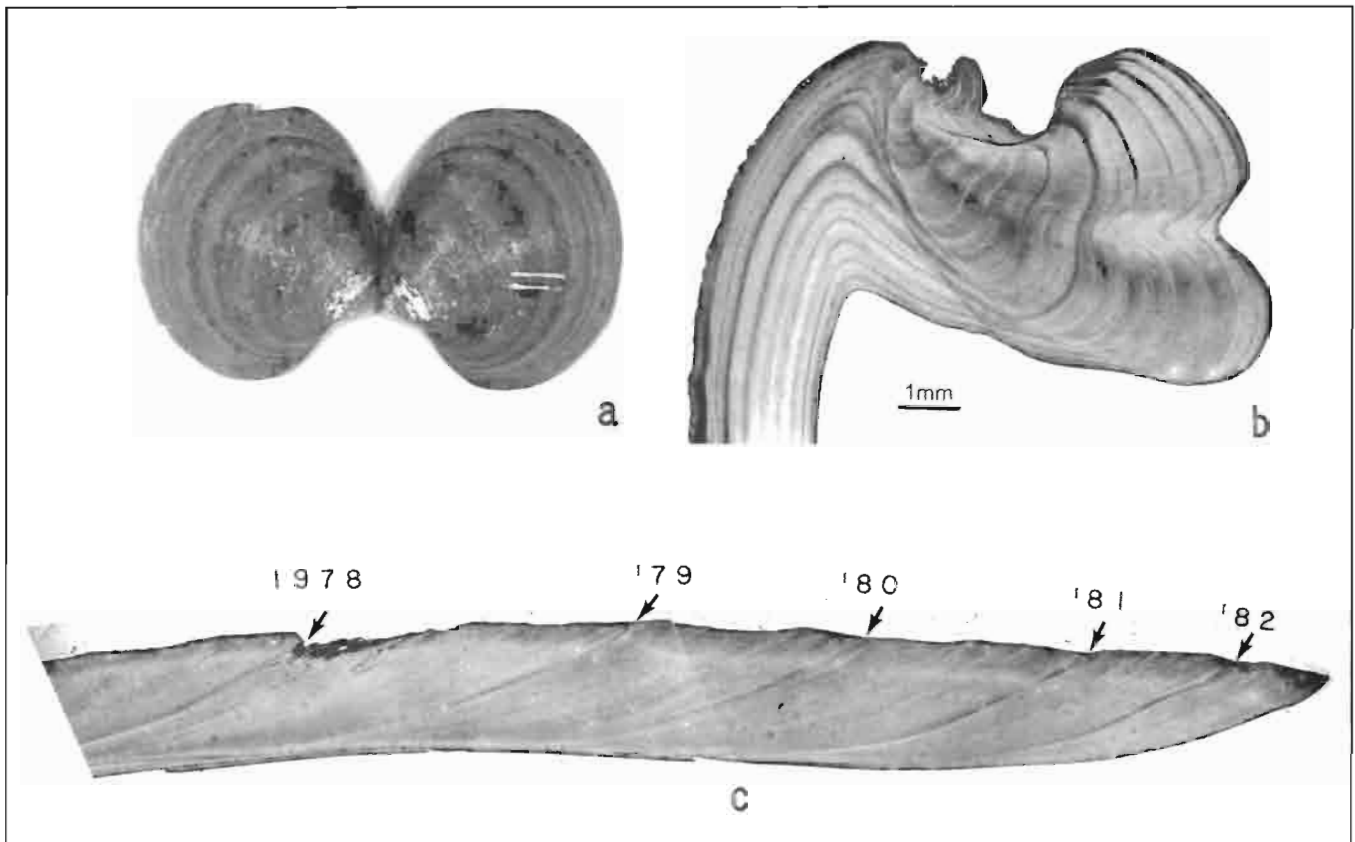
Figure 4—a) A 62-mm shell length ocean quahog, Arctica islandica , marked in 1978 and recaptured in 1983. Paired parallel notches clearly delimit growth (estimated to be 14.4 mm) after marking. b) Eleven annuli are shown in the photomicrograph of the clam's hinge tooth. These corresponded to the same number of annuli found in the valve. c) Replicate peel photomicrograph of the sectioned ventral valve margin showing an annulus that had formed soon after marking and four annuli formed thereafter. Each annulus is identified by the year of its formation. A millimeter scale applies to peel replicate photomicrographs b and c.
