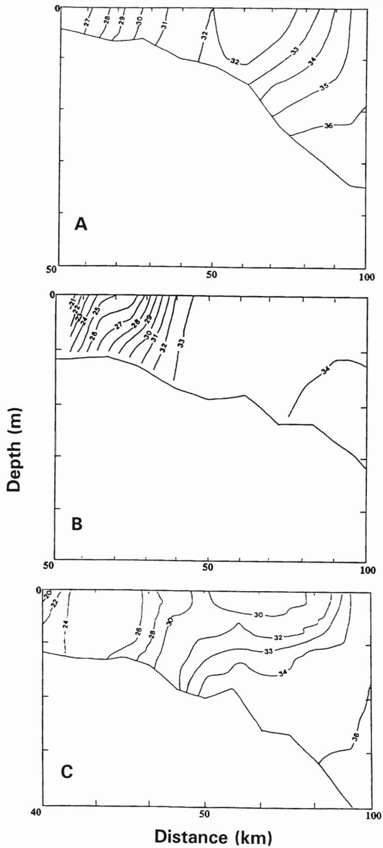
Figure 3 Salinity contours of Line 4 for the (A) May 1992, (B) May 1993, and (C) May 1994 LATEX hydrography cruises.
