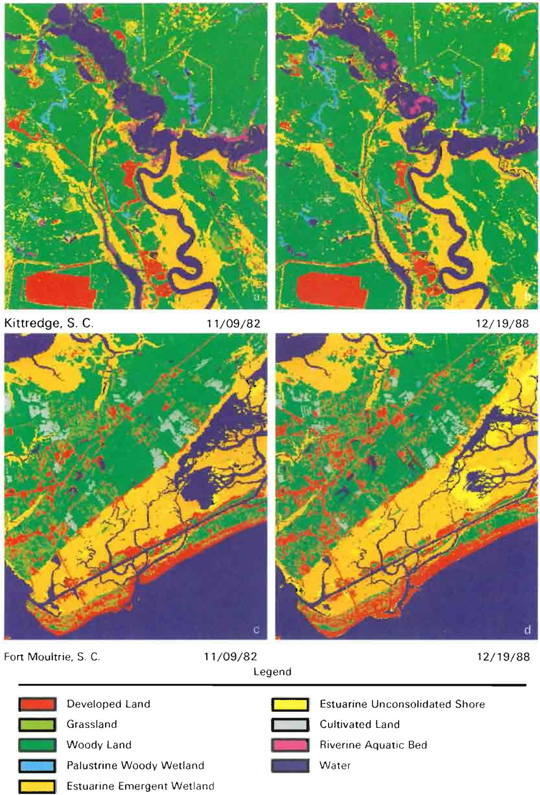
Figure 7 Multiple-date land-cover classification maps: (a and b) Kittredge, S. C., study area, produced from 9 Nov 1982 and 19 Dec 1988 Landsat TM data. (c and d) Fort Moultrie, S. C., study area, produced from 9 Nov 1982 and 19 Dec 1988 Landsat TM data (Jensen et al., 1993a).
