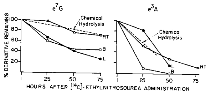
FIGURE 6. Stability of e^7G (7-ethyl G) and e^3A (3-ethyl A) in DNAs in ethylnitrosourea-treated 10-day-old BD IX rats (30), as compared to the chemical stability in vitro (7): (—) rate of chemical hydrolysis at pH 7, 37°C; (○) brain; (●) liver; (Δ) other tissues, pooled.
