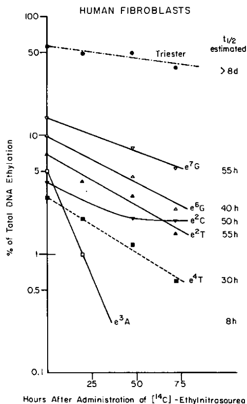
FIGURE 4. Amounts of [ ^{14}\text{C} ]ethyl products from ethyl nitrosourea-treated mammalian cells, prelabeled with ^3\text{H} . The initial proportion of total ethylation is shown on the log scale. All values have been corrected for cell division. The estimated t_{1/2} of derivatives is shown in the figure. Adapted from Bodell et al. (14).
