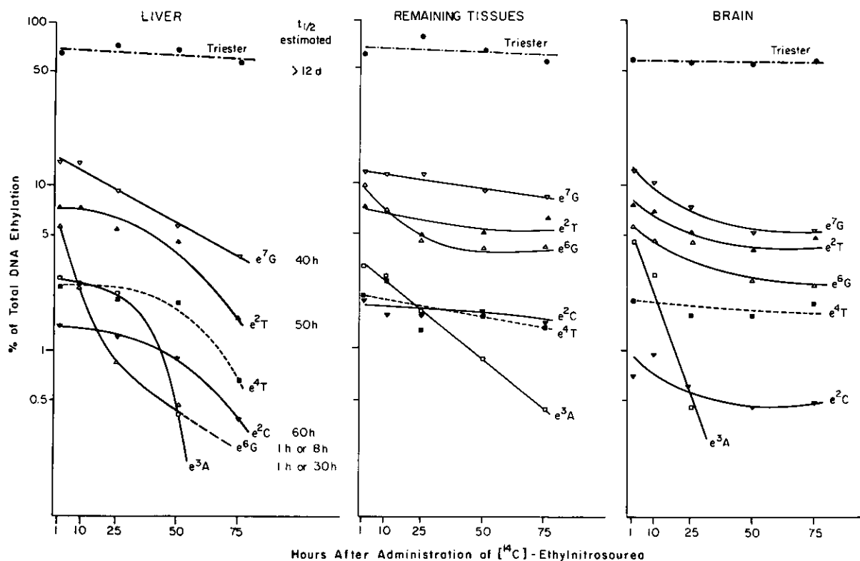
FIGURE 5. Amounts of ethyl derivatives at 1, 10, 25, 50, and 75 hr after administration of [ ^{14} C]ethylnitrosourea to 10-day-old BD IX rats. The number of ethyl groups bound in various organs was 1.3–3 per 10^6 DNA-P (30): (left) liver DNA; estimated half-lives of each derivative are shown in the figure; (middle) pooled DNA from spleen, lung, thymus, muscle, and intestine; (right) brain DNA.
