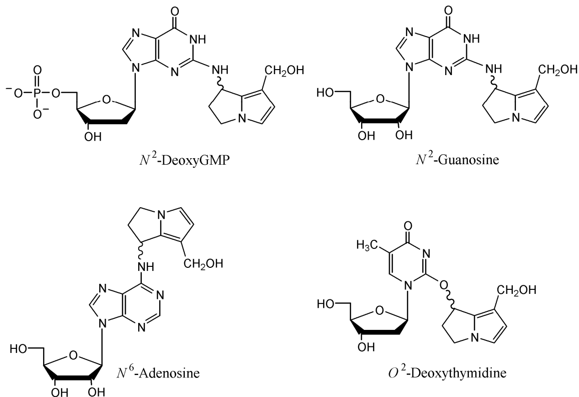
Figure 5-4. Alkylation of nucleosides and nucleotides by dehydronecine
