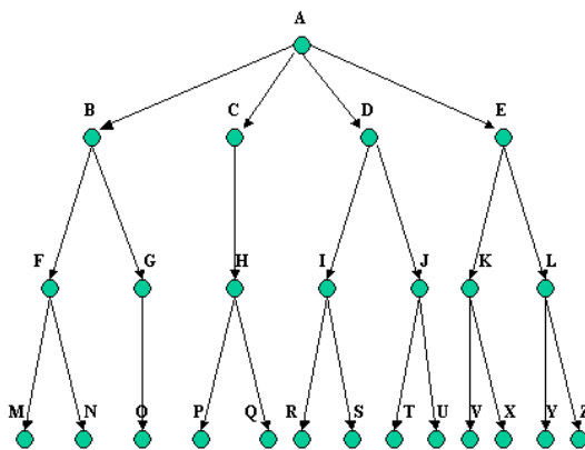
Figure 1. Hyperlink tree
