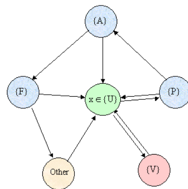
Figure 4. Constraint graph
