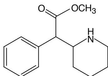
Figure 1. Chemical structure of methylphenidate (C 14 H 19 NO 2 )
