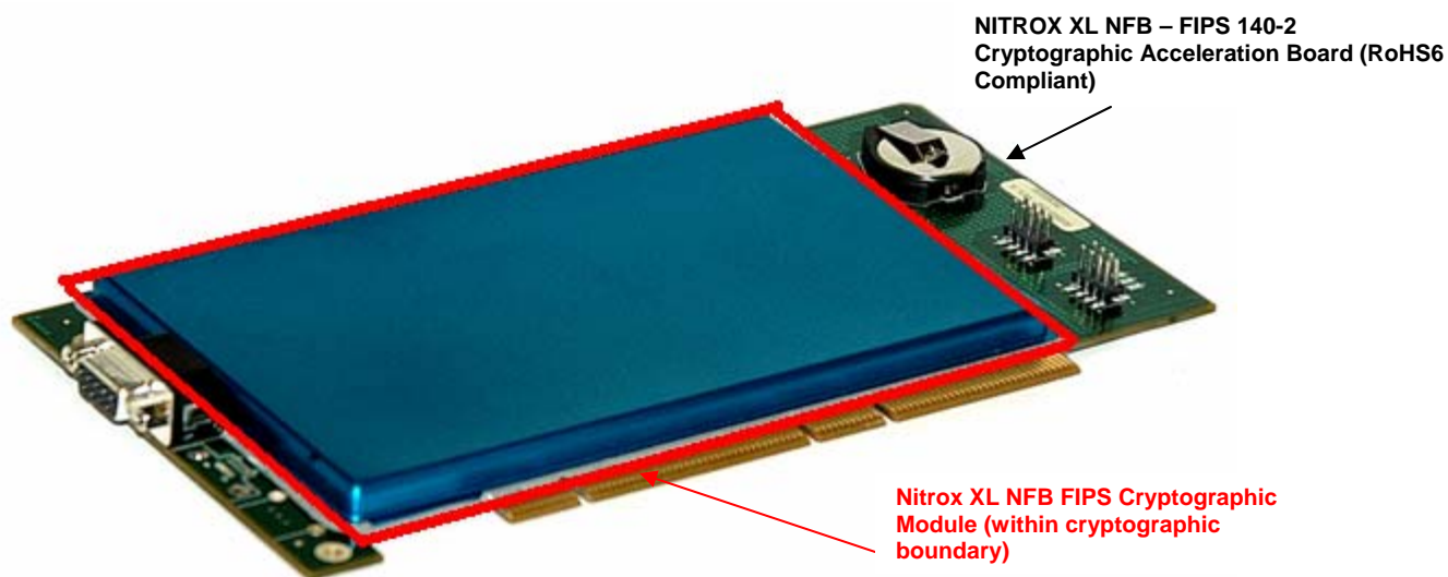
Figure 2-1. Nitrox XL NFB FIPS Cryptographic Module
