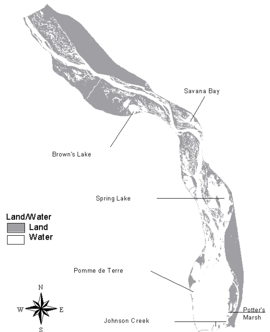
Figure 4. Pool 13, Upper Mississippi River, transect locations for the 1992 monitoring of submersed aquatic vegetation for the Long Term Resource Monitoring Program.
