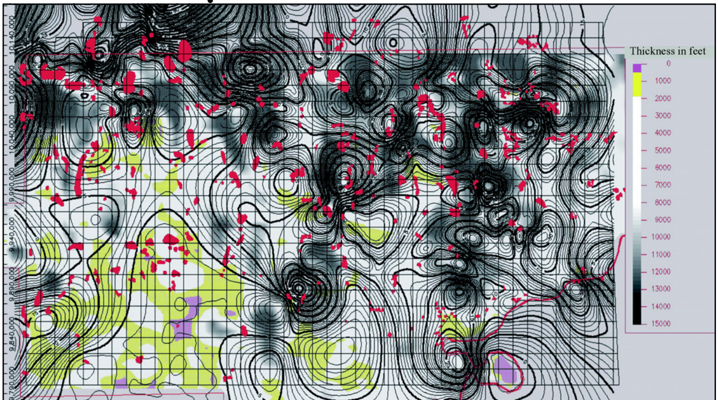
• An example of the combination of data types necessary for methane hydrate assessment by MMS. • This example includes: sand percent isopach, total sediment thickness (indicated by color bar at right), and the location of ocean bottom anomalies (in red). The data is from the Green Canyon Area of the Gulf of Mexico. The Sigsbee Escarpment is delineated by the red line in the lower right corner.
