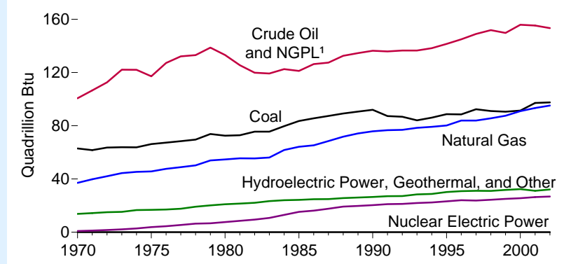
Figure 58. World Primary Energy Production By Source
