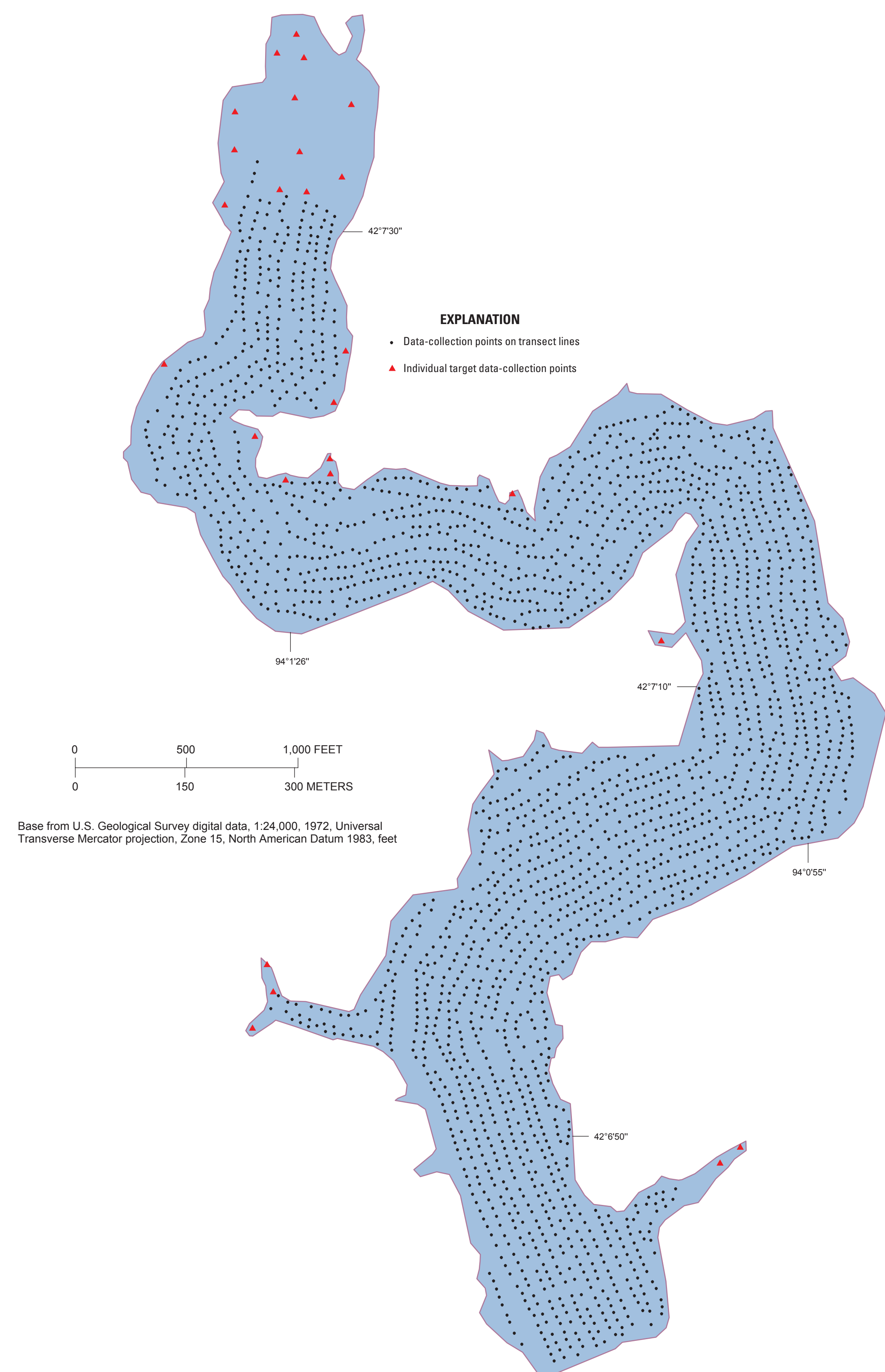
Figure 1. Data-collection points used to construct bathymetric contours.
