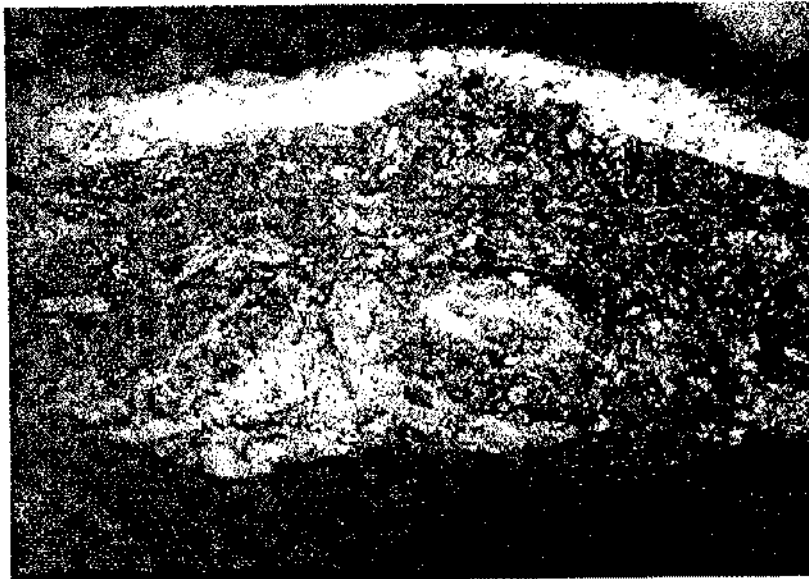
Figure 1. LOM macrograph of encrustation cross section.
