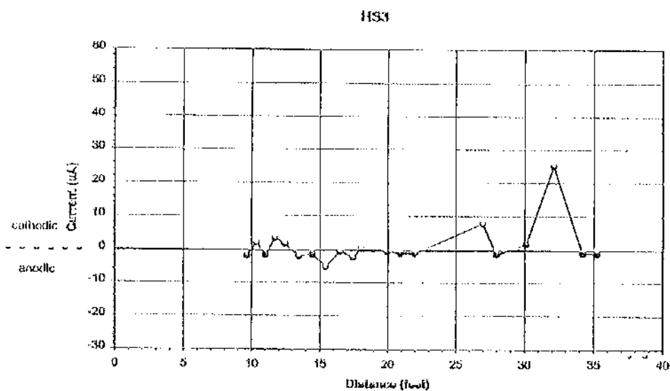
Figure 5. Surface current flux for transect H1S.
