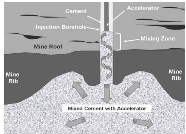
Figure 2. Downhole depiction of a conventional remote mine seal installation.
