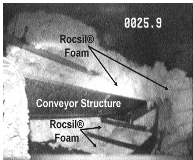
Figure 10. Screen capture from video showing completed seal. Note numbers in the upper right hand corner of the image indicate to borehole depth.
