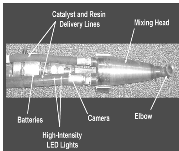
Figure 11. Improved foam delivery system that combines the downhole mixing head and the camera system.
