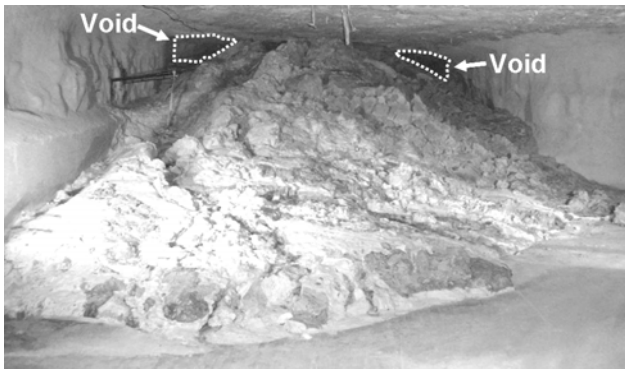
Figure 3. Cement-based remotely installed mine seal. Note open void areas.
