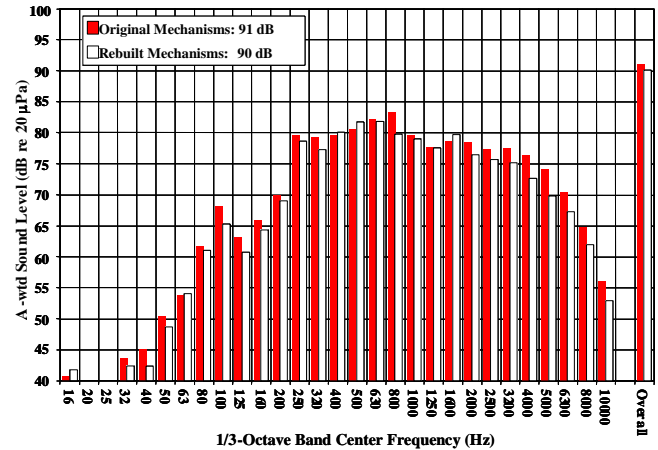
Figure 17. A-wtd 1/3-octave band sound levels for vibration only operation with original and rebuilt mechanisms.
