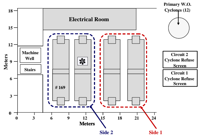
Figure 2. Overhead view of test area.
