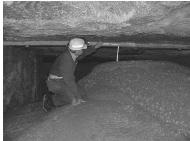
Figure 5. Underground view of bulk fill material for seal No. 1.
