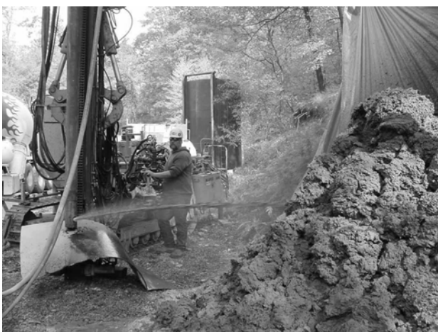
Figure 10. Surface test of spray grout system.
