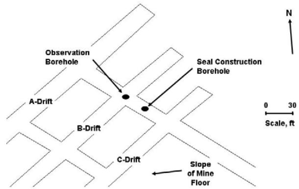
Figure 2. Underground layout of the seal construction site.
