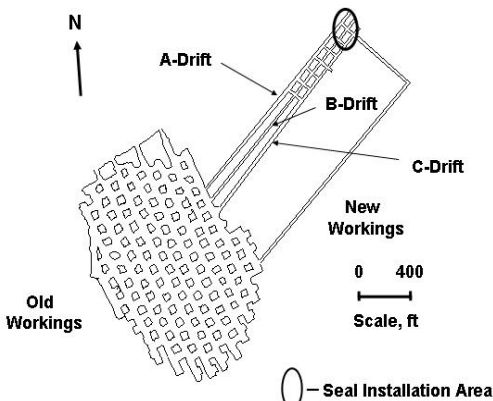
Figure 1. Layout of the Lake Lynn Laboratory Mine.
