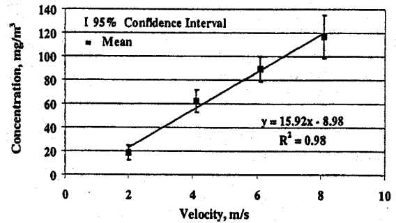
Figure 3. Relationship between total dust concentration and air velocity.
