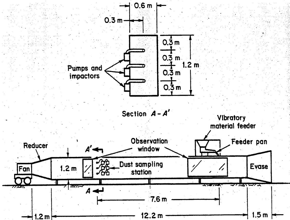
Figure 2. Dust entrainment tunnel schematic.
