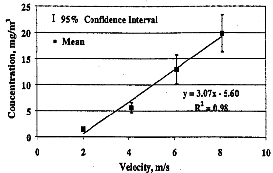
Figure 4. Relationship between respirable dust concentration and air velocity.
