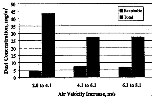
Figure 6. Rise in dust concentrations for each air velocity increase
