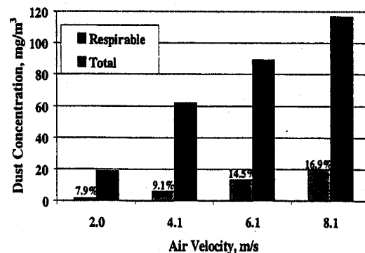
Figure 5. Percent of respirable dust in impactor samples at each air velocity.
