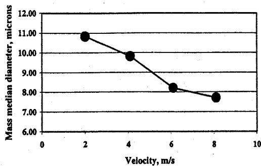
Figure 8. Mass median diameter for each test velocity.
