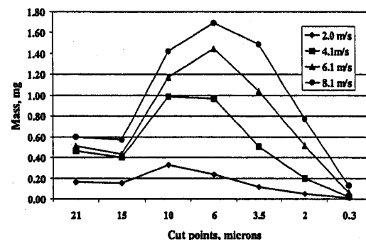
Figure 7. Average dust distribution by impactor cut points.
