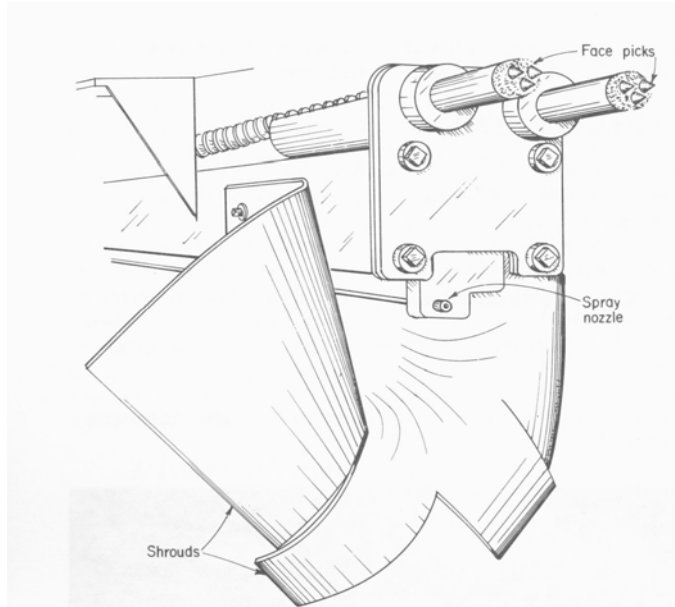
Figure 3. External boom mounted water spray.
