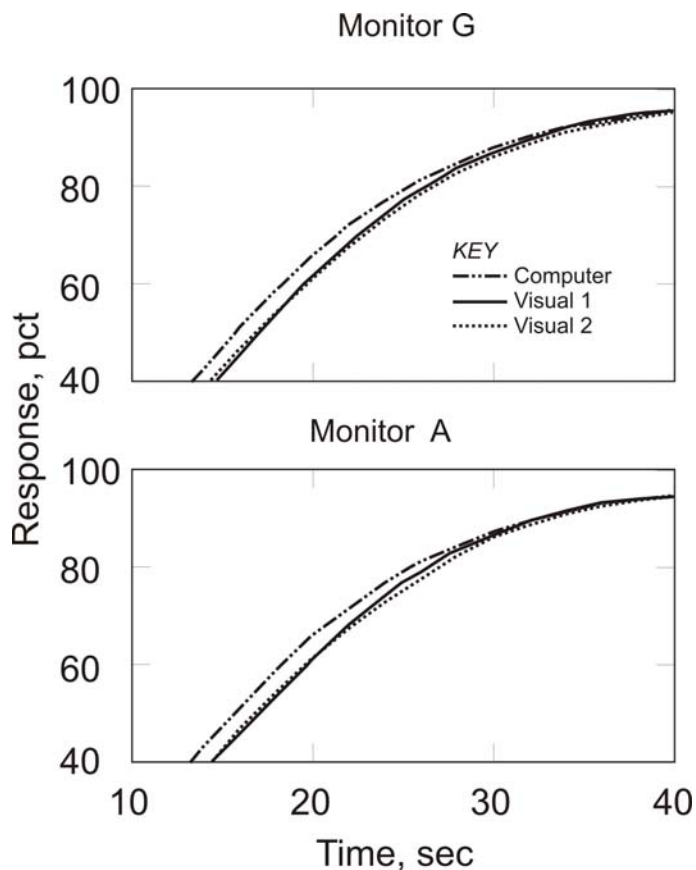
Figure 4. Comparison of response time data obtained with computer and visual observations.
