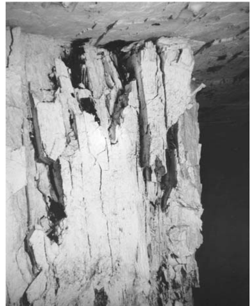
Figure 1. Vertical coal pillar slabs associated with face cleat.
